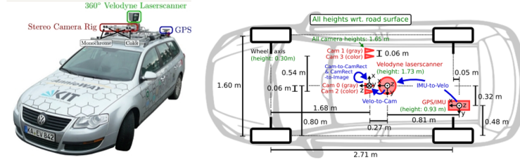
Figure 6: KITTI data-collection platform, reprinted from benchmark materials associated with Geiger et al. [4]. All experiments in this report are based on archived KITTI Tracking results.
