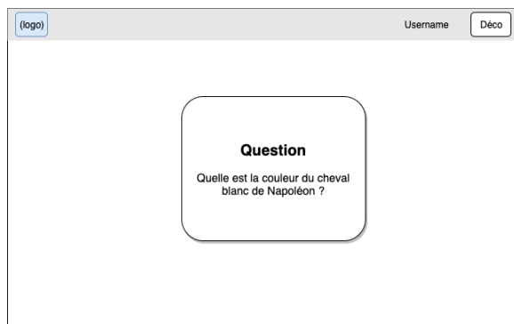
Presentquestion
