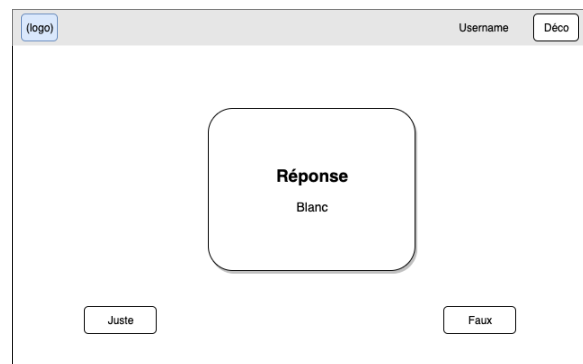
Presentresponse
