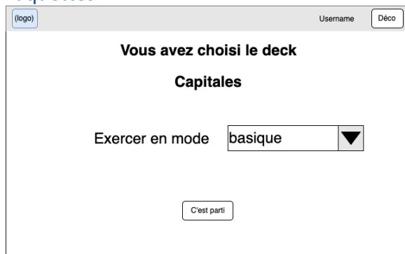
Start
