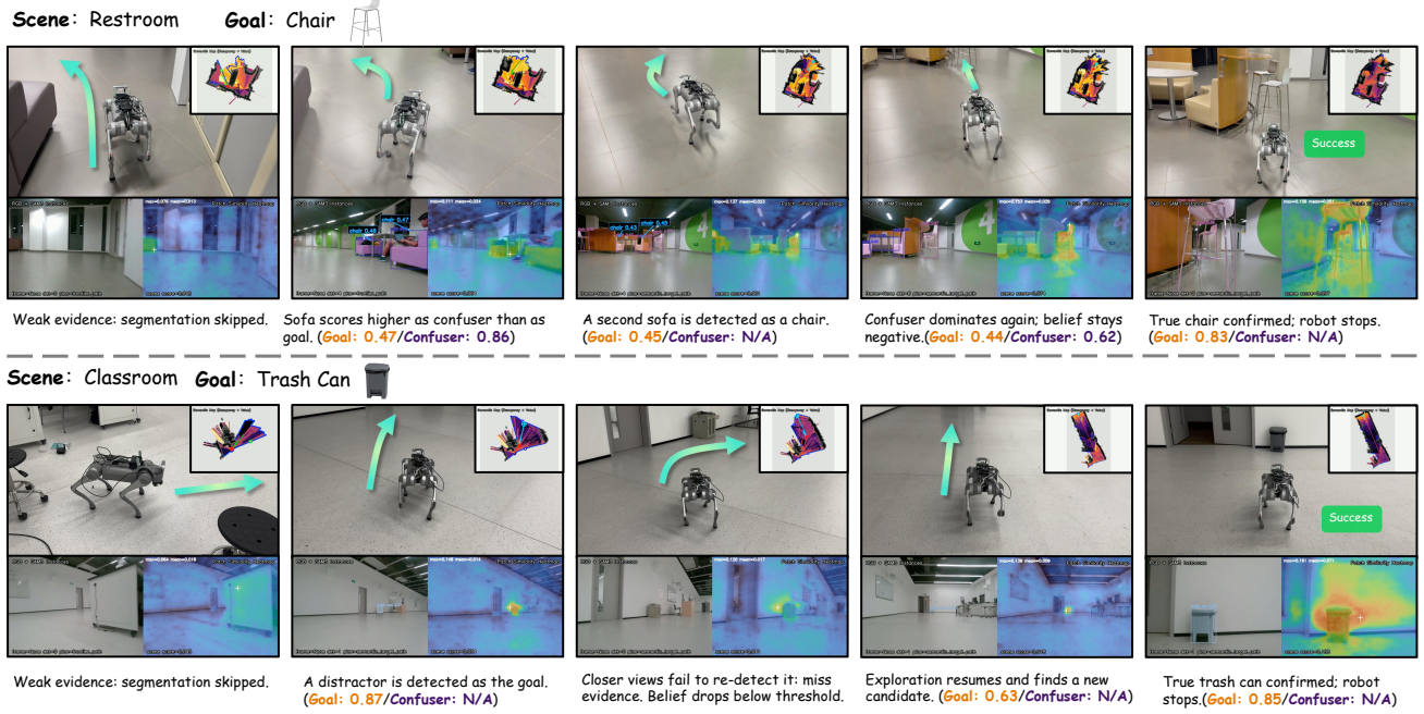
Fig. 4. Real-world trials on a Unitree Go2. Top: confuser evidence rejects two sofas while searching for a chair. Bottom: miss evidence withdraws a distractor that fails to reappear at close range, and the robot then reaches the true object.
