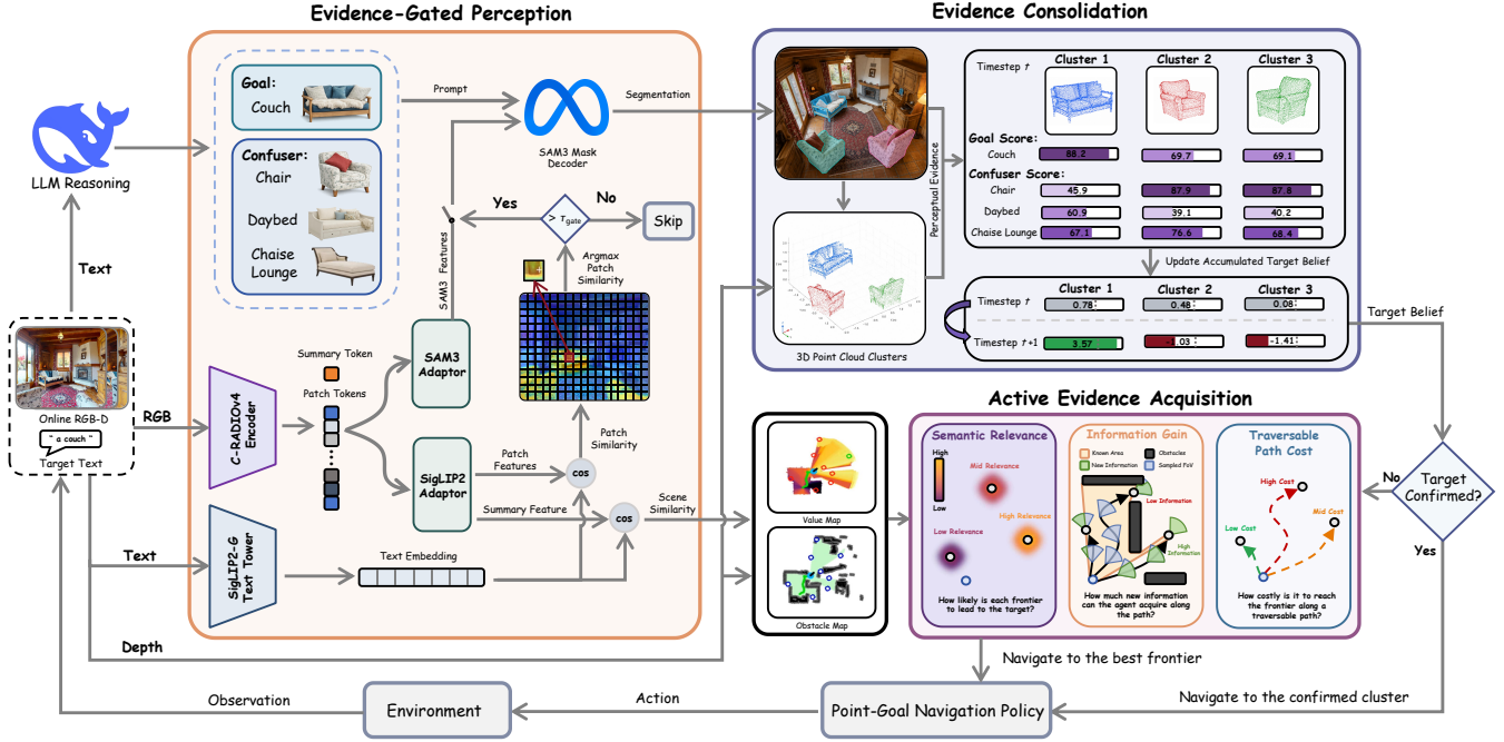
Fig. 2. Framework of AECNav. AECNav comprises three modules: evidence-gated perception, which uses a shared C-RADIOv4 encoder to score scene relevance and trigger SAM3 only when a probable target is observed; evidence consolidation, which back-projects detections into 3D clusters and updates their log-odds beliefs using goal, confuser, and miss evidence; and active evidence acquisition, which selects frontiers by jointly considering semantic relevance, information gain, and traversal cost until a target cluster is confirmed. Confuser categories are generated offline by an LLM.
