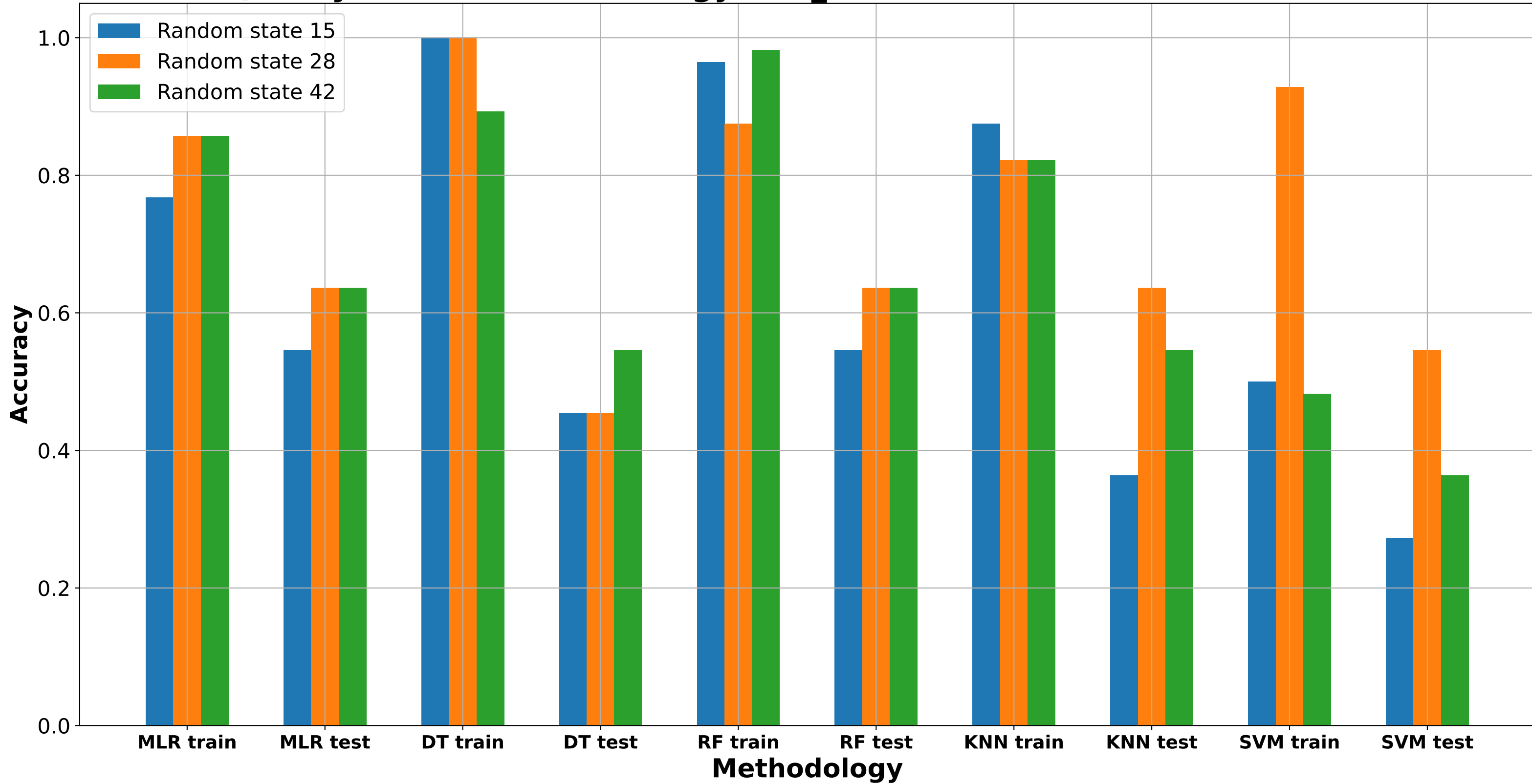
Quality of each methodology - ee_acc max number of features: 11
