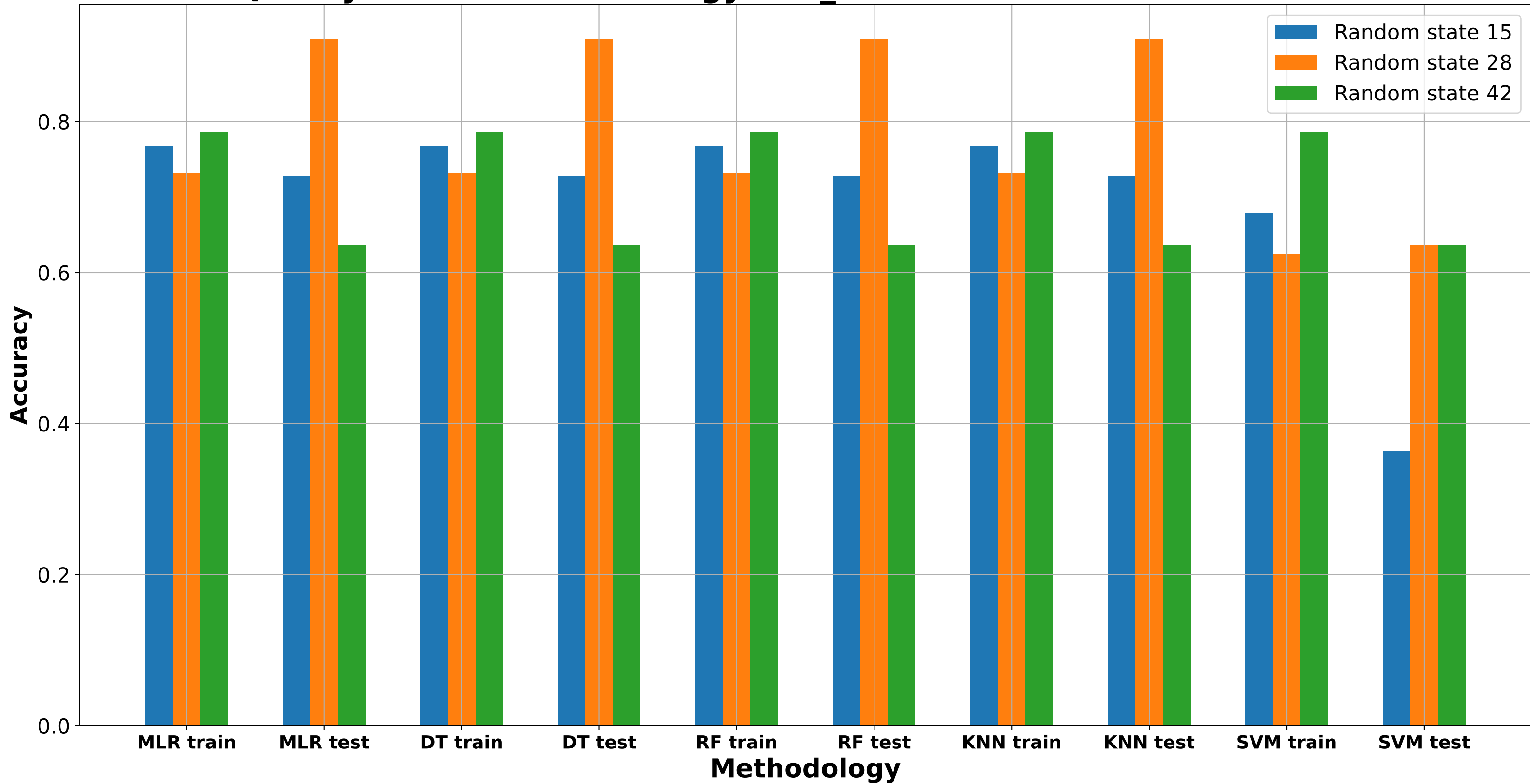
Quality of each methodology - ee_acc max number of features: 2
