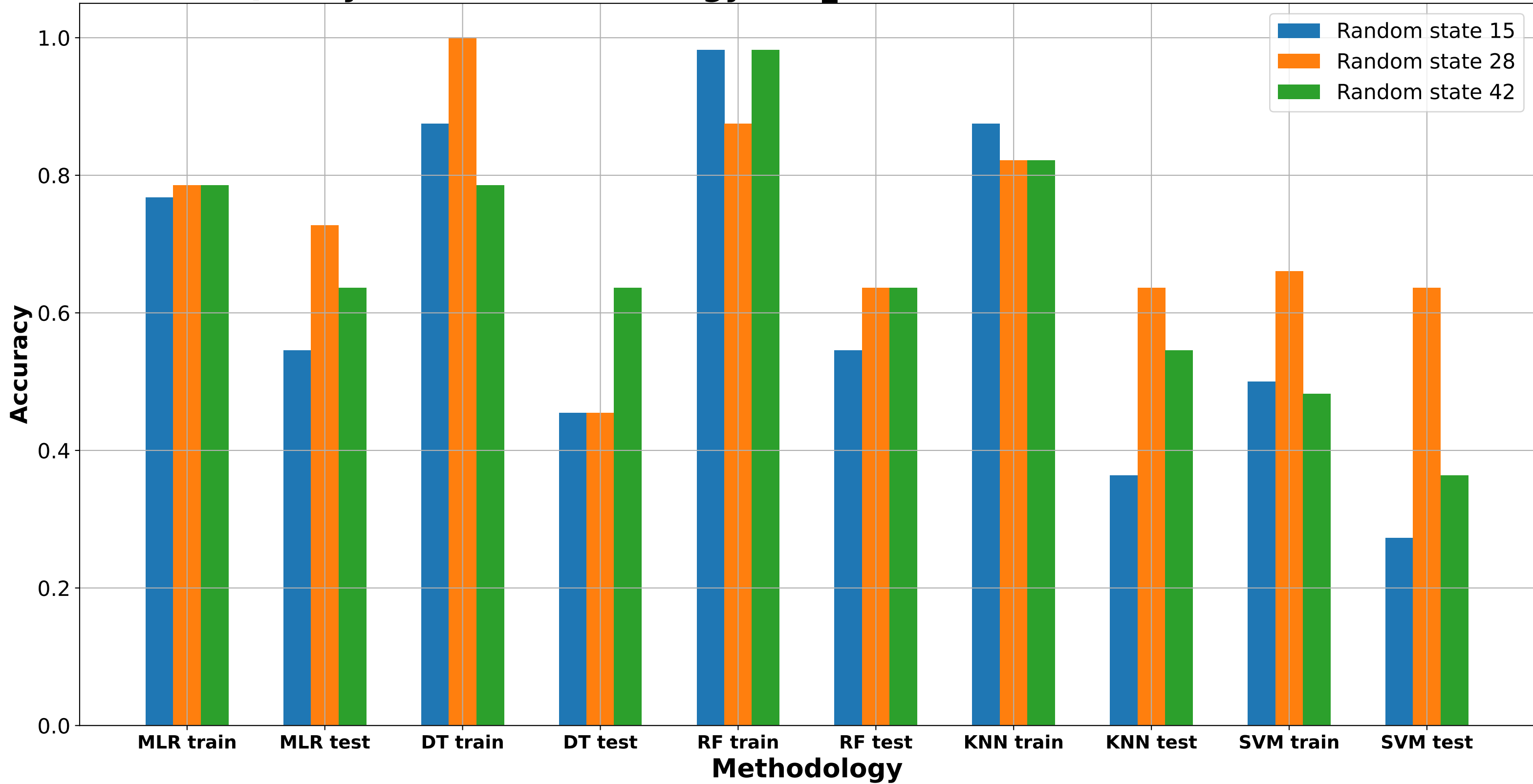
Quality of each methodology - ee_acc max number of features: 7
