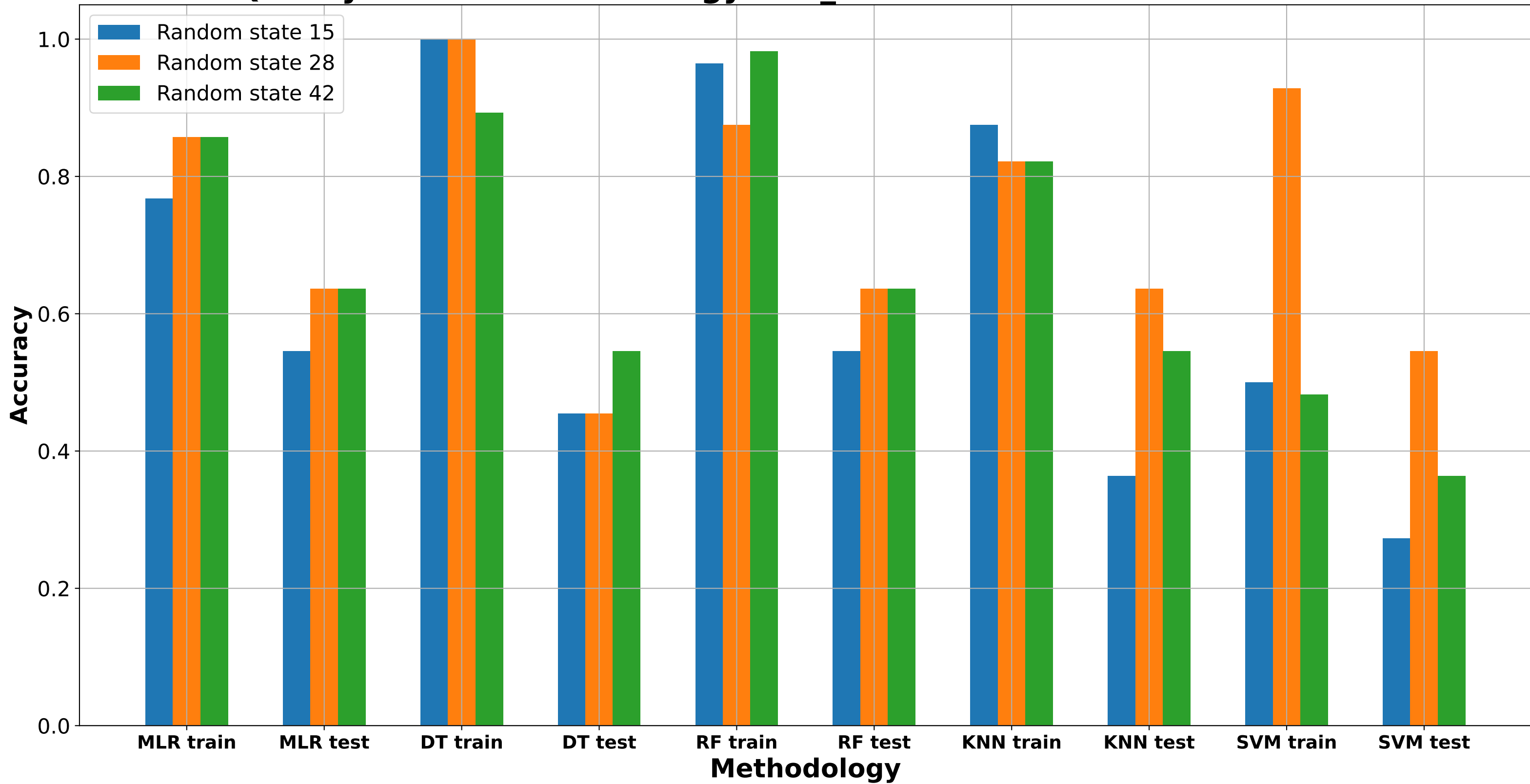
Quality of each methodology - ee_acc max number of features: 9
