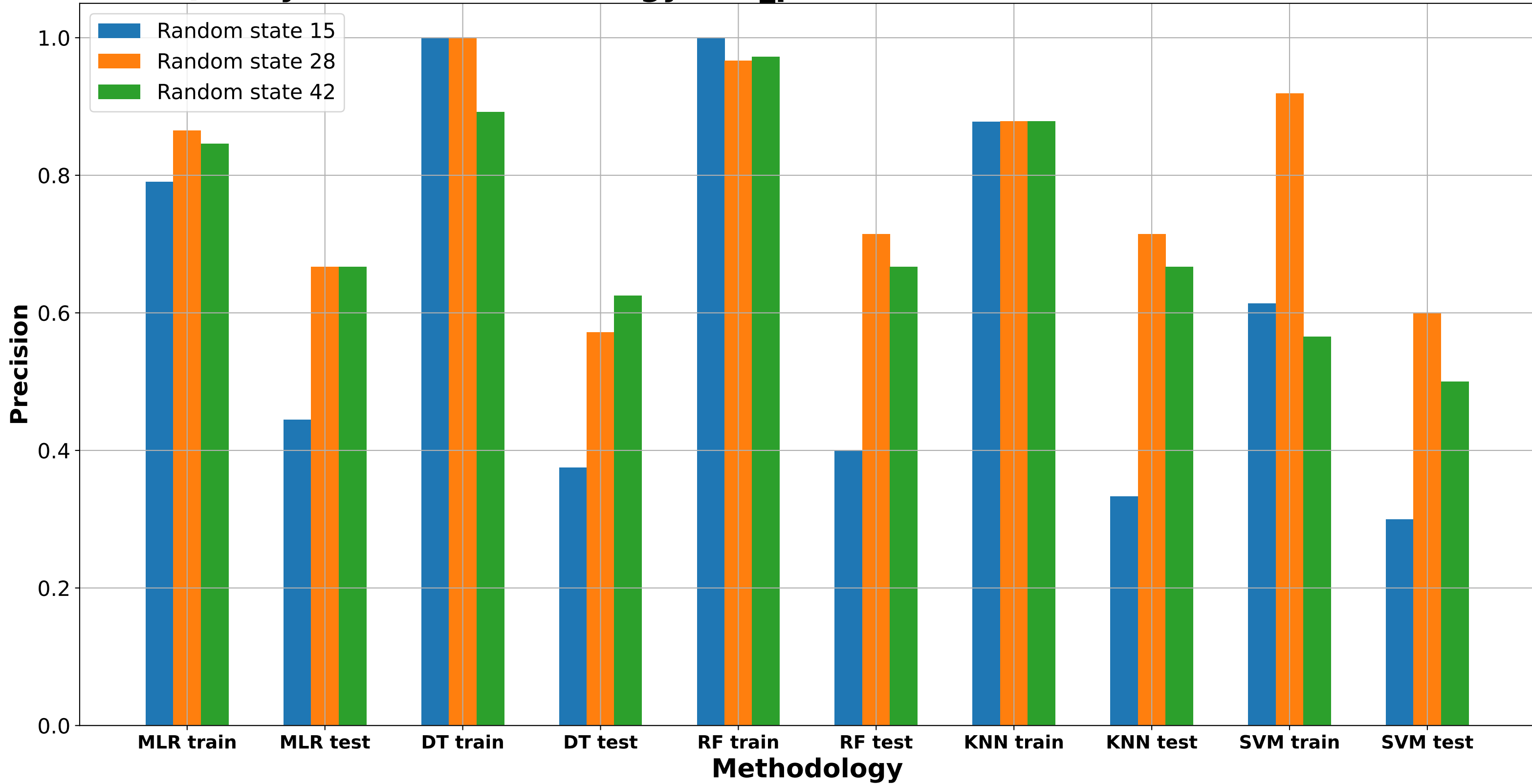
Quality of each methodology - ee_precision max number of features: 10
