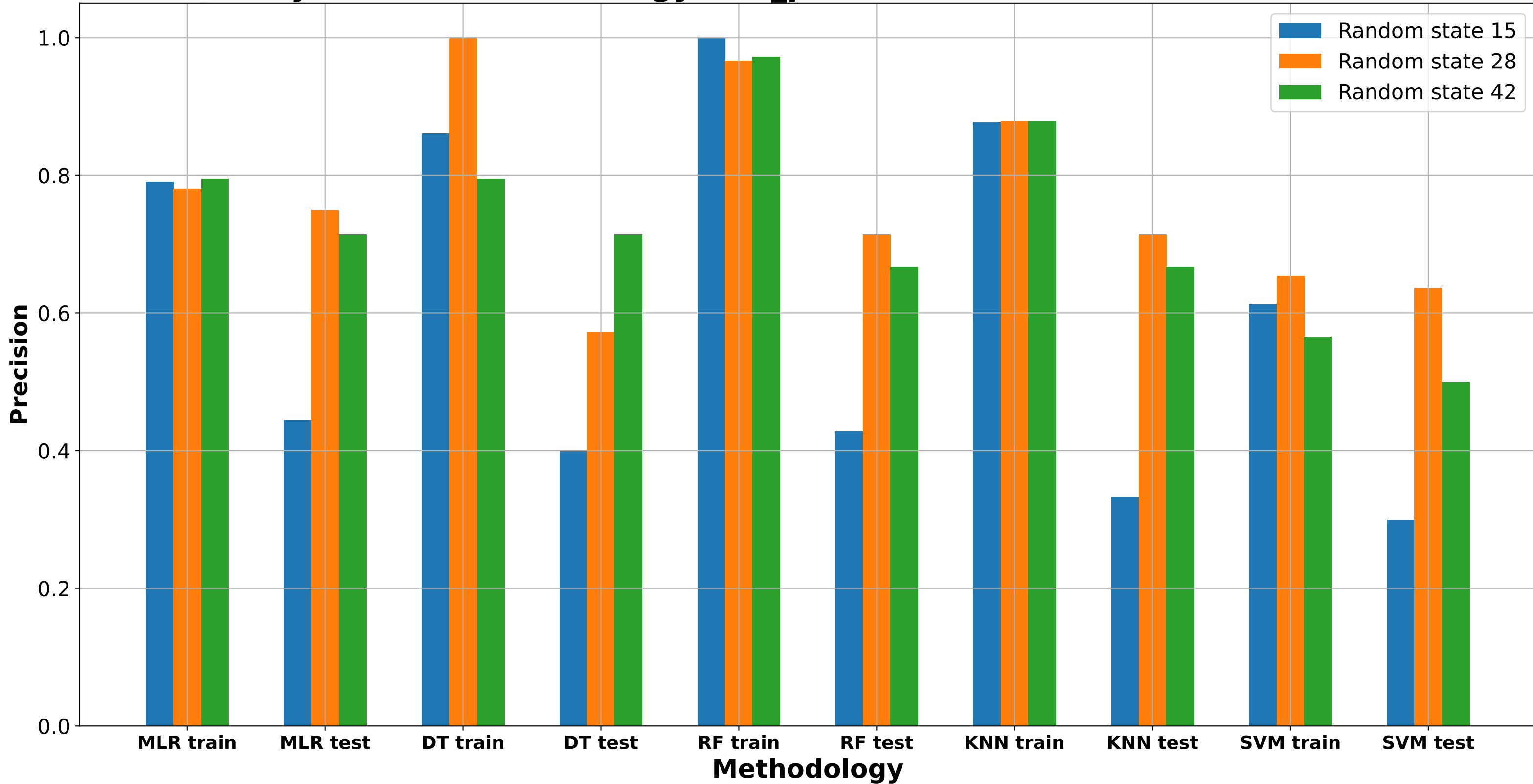
Quality of each methodology - ee_precision max number of features: 6
