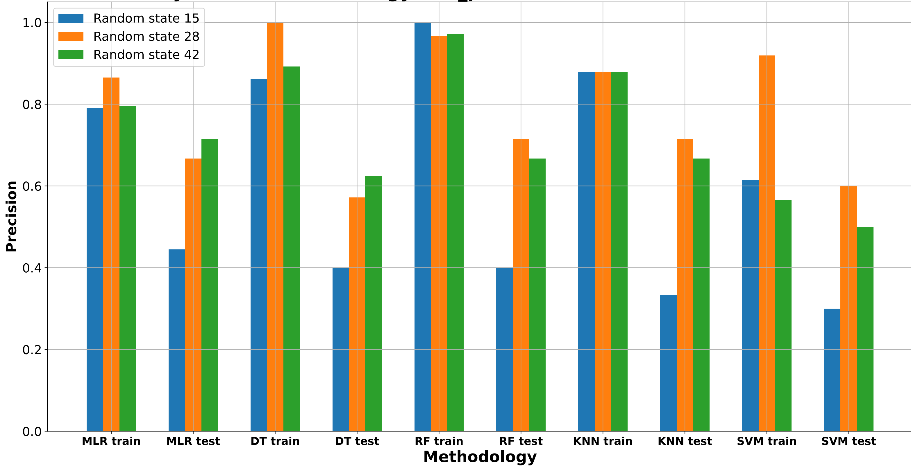
Quality of each methodology - ee_precision max number of features: 8
