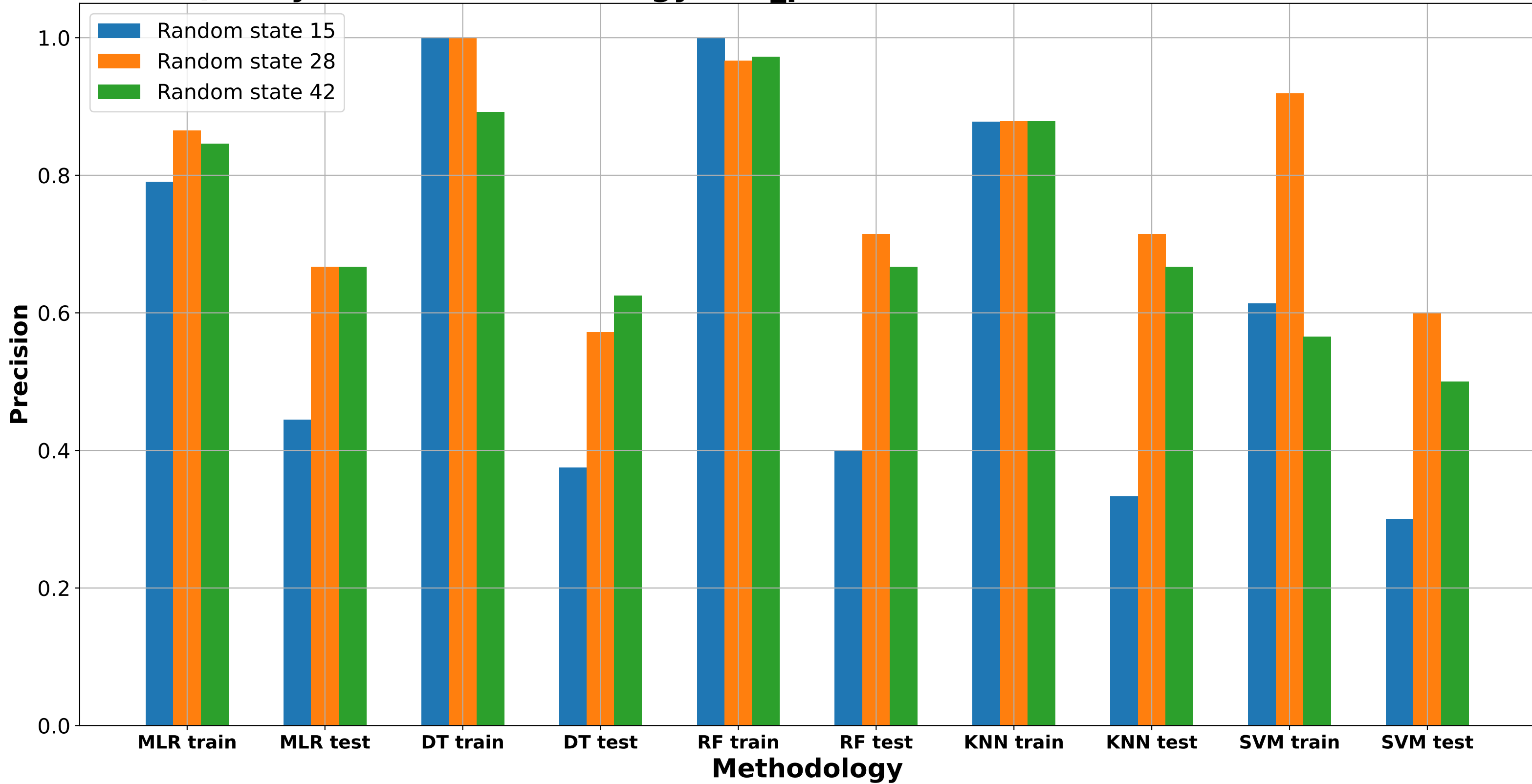
Quality of each methodology - ee_precision max number of features: 9
