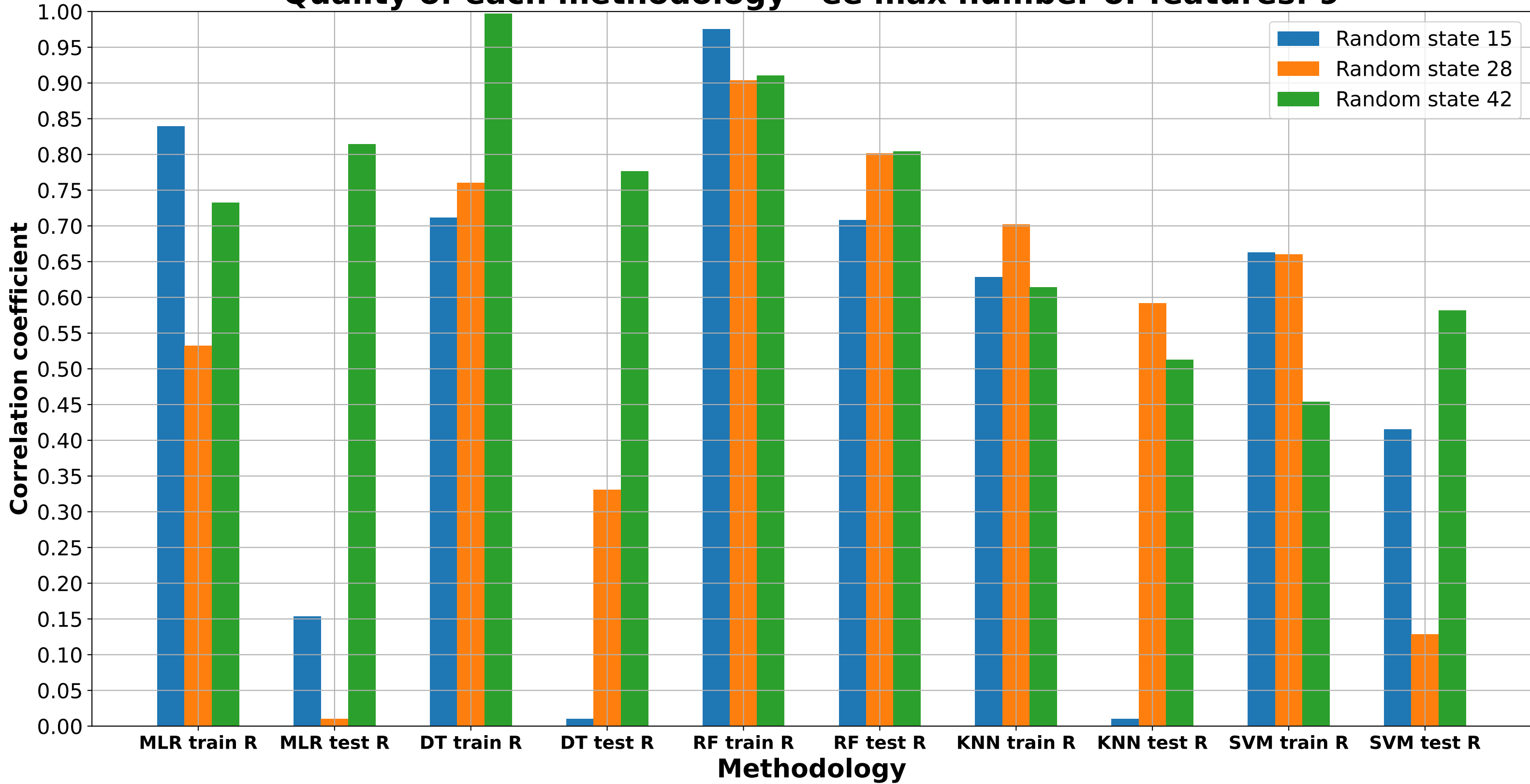
Quality of each methodology - ee max number of features: 9
