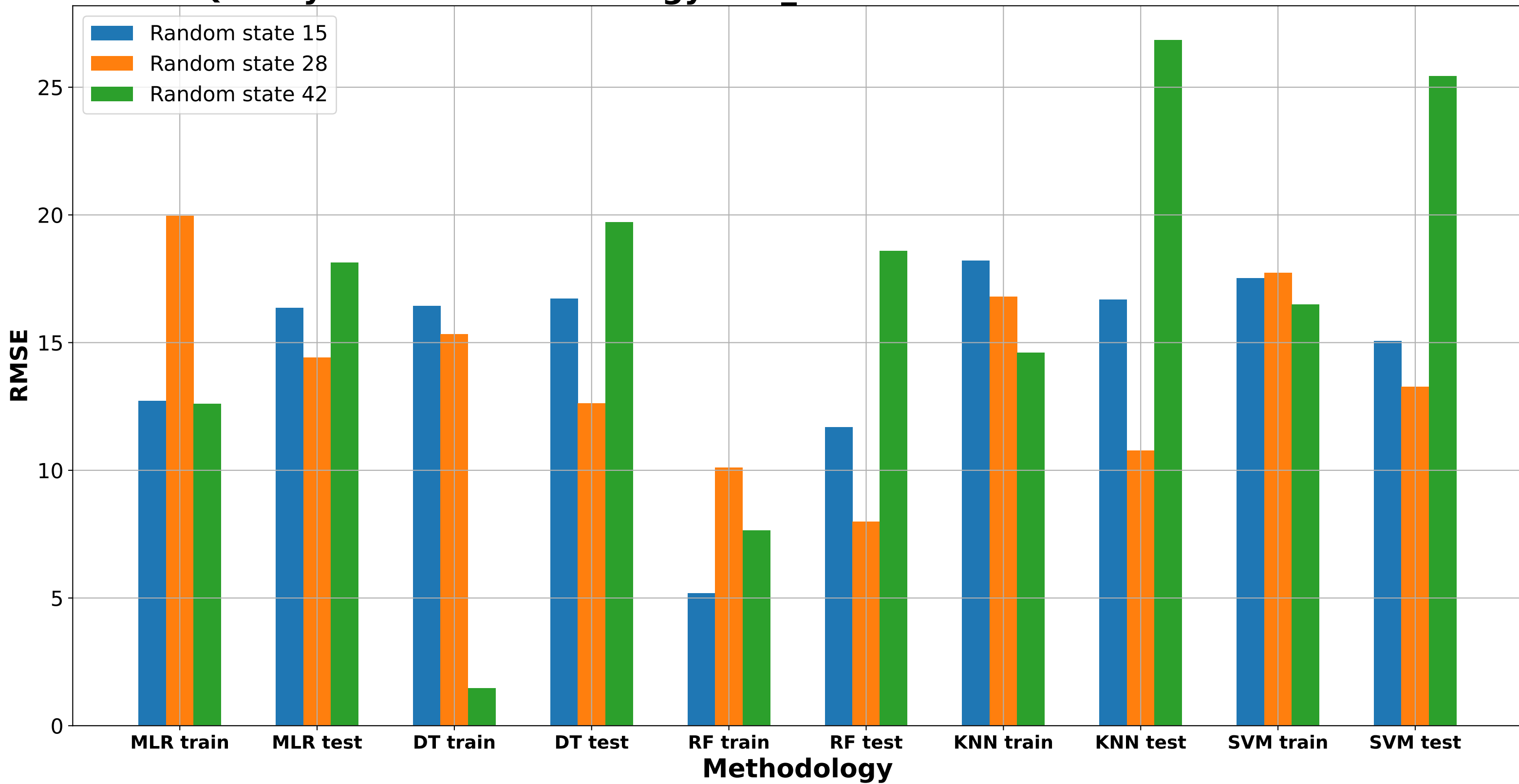
Quality of each methodology - ee_RMSE max number of features: 11
