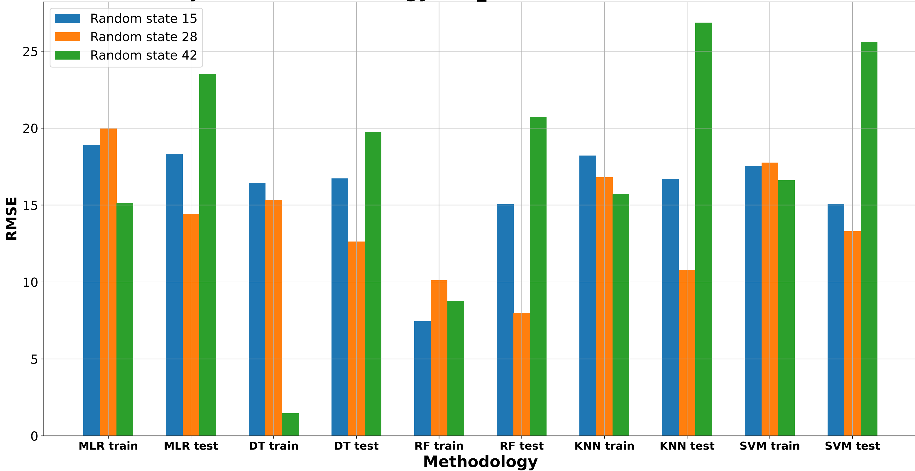
Quality of each methodology - ee_RMSE max number of features: 7
