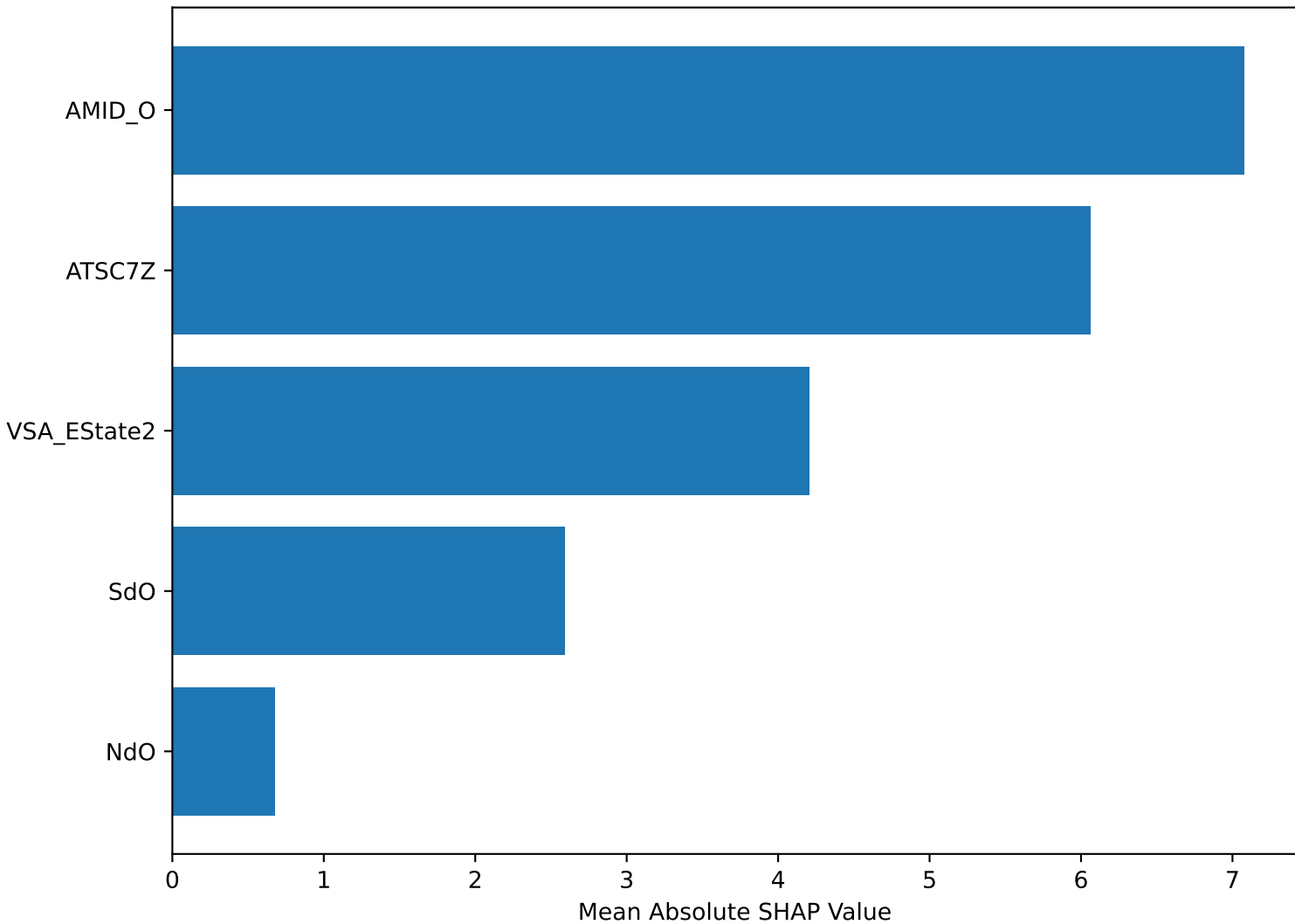
Global Feature Importance in RandomForestRegressor (SHAP)
