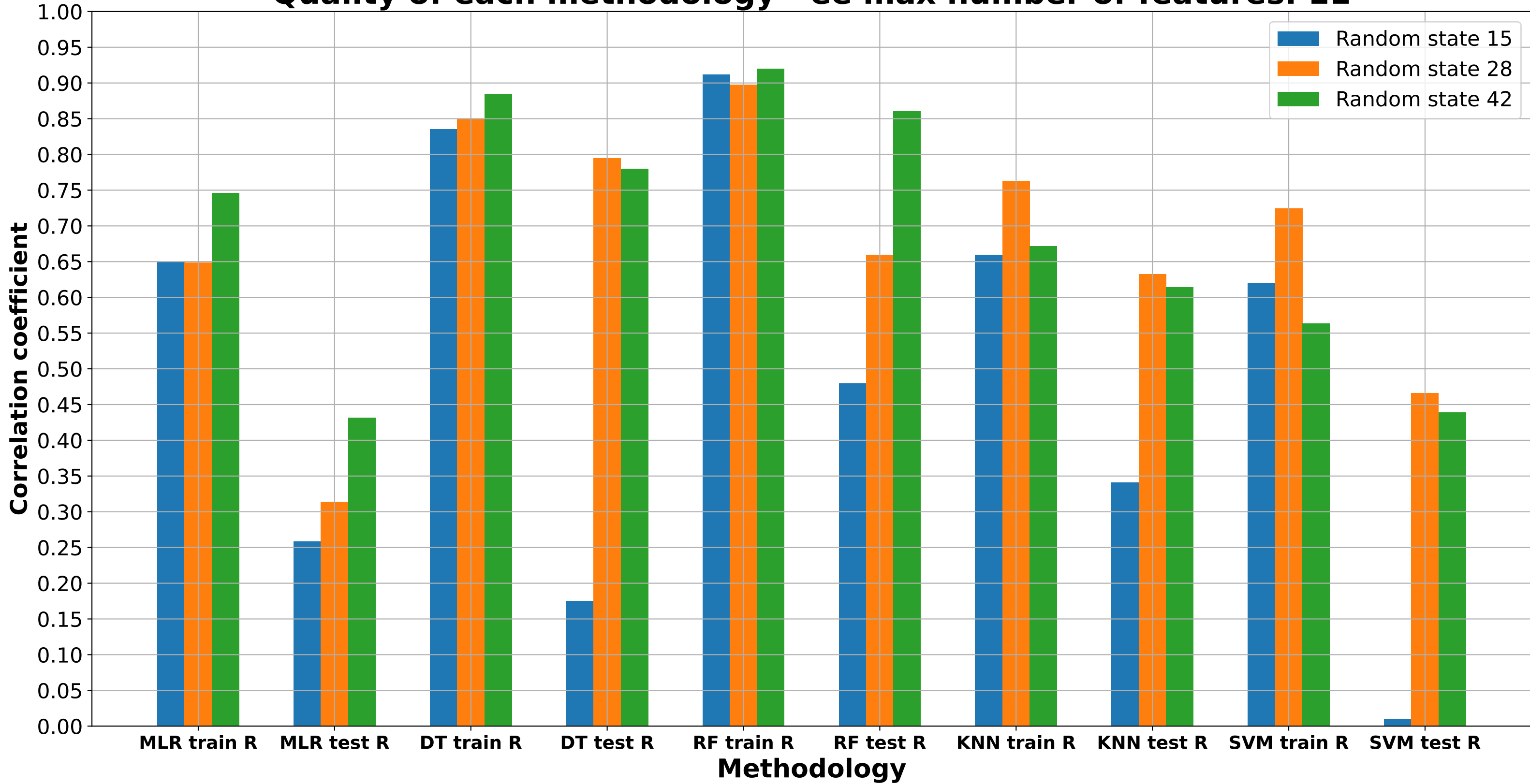
Quality of each methodology - ee max number of features: 11
