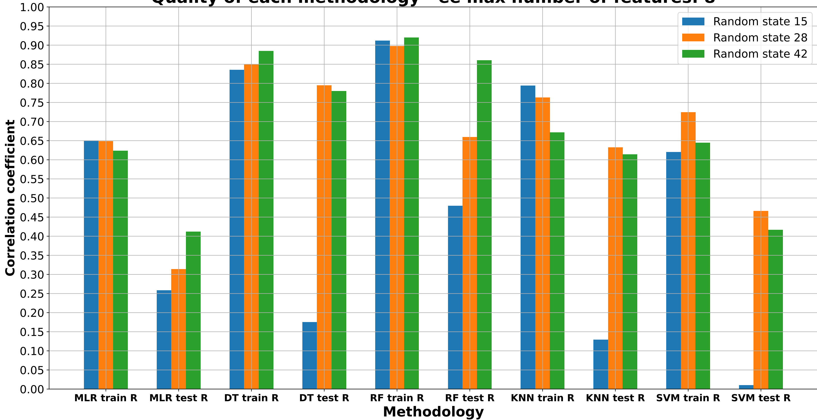
Quality of each methodology - ee max number of features: 8
