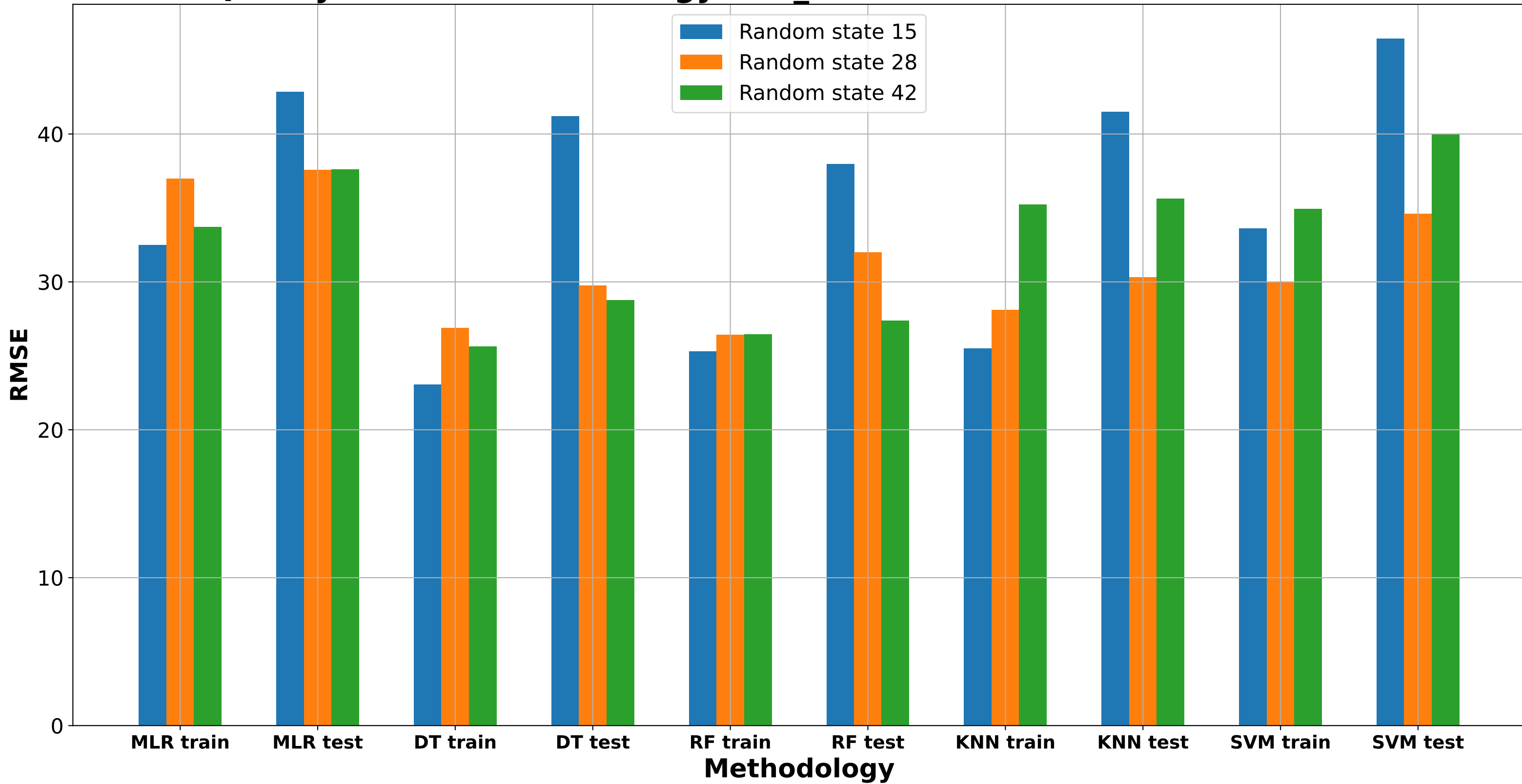
Quality of each methodology - ee_RMSE max number of features: 2
