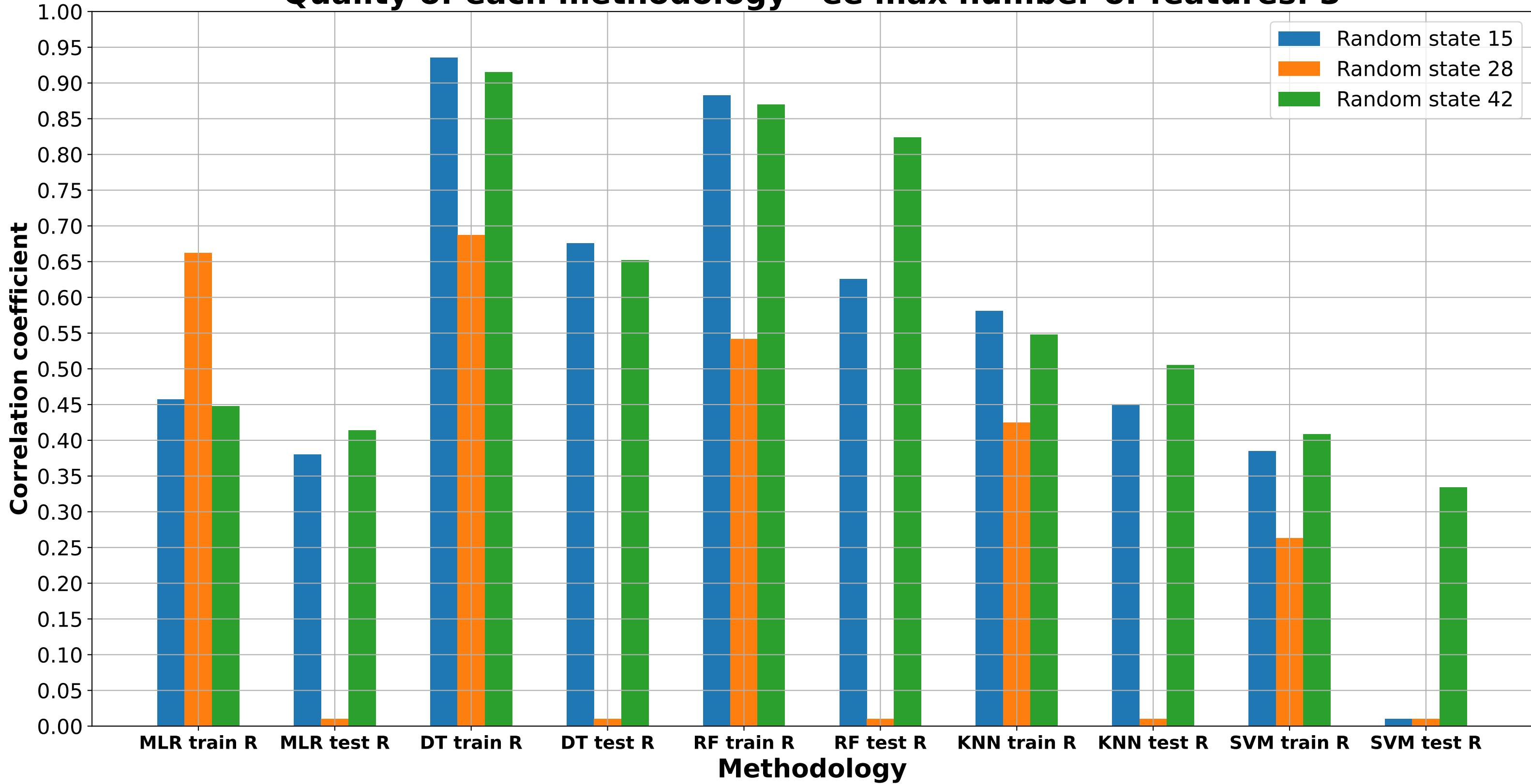
Quality of each methodology - ee max number of features: 3
