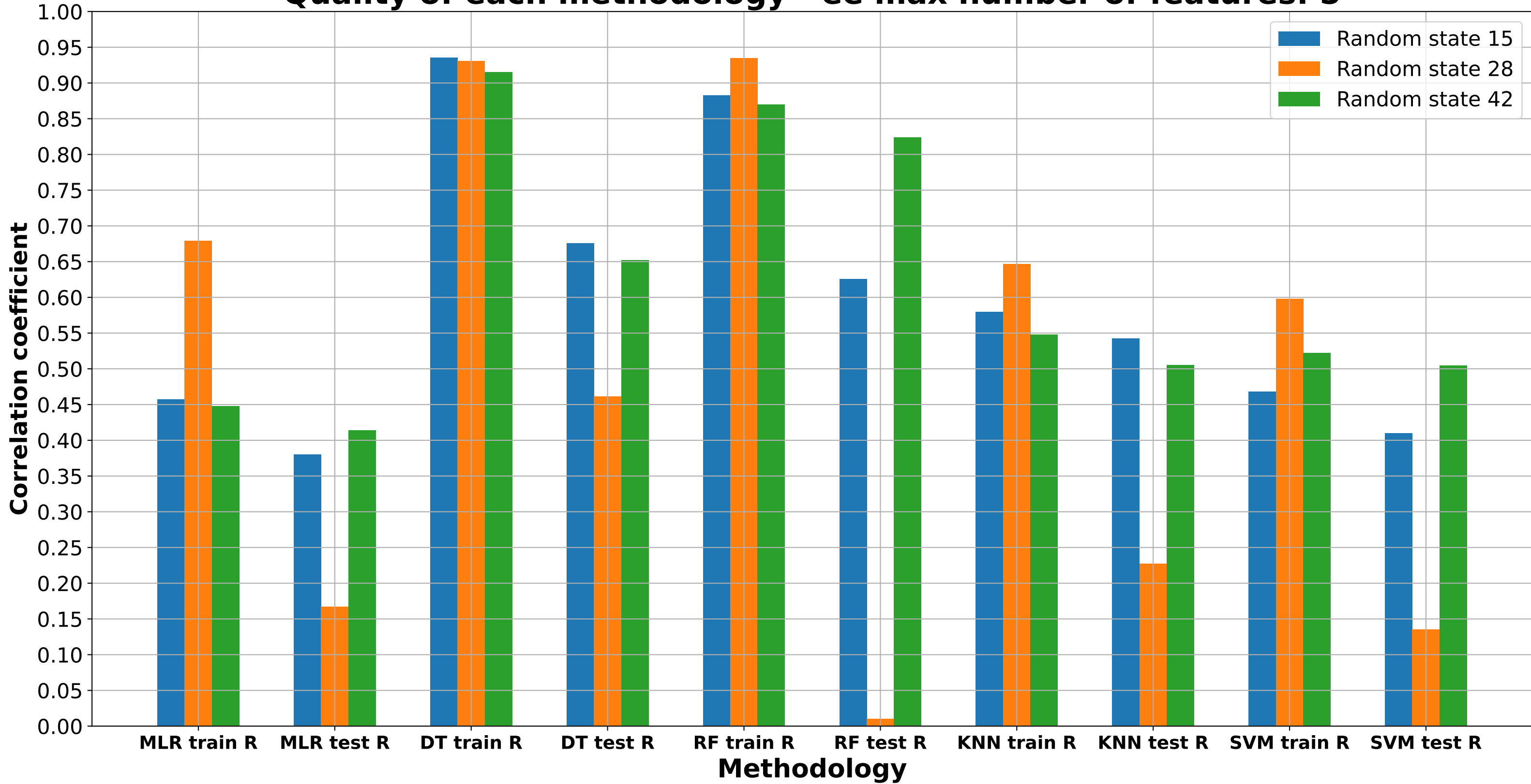
Quality of each methodology - ee max number of features: 5
