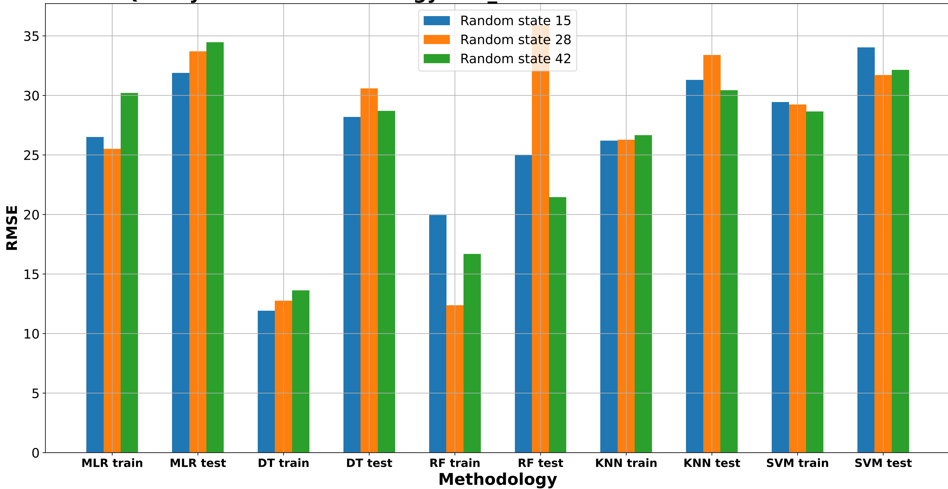
Quality of each methodology - ee_RMSE max number of features: 12
