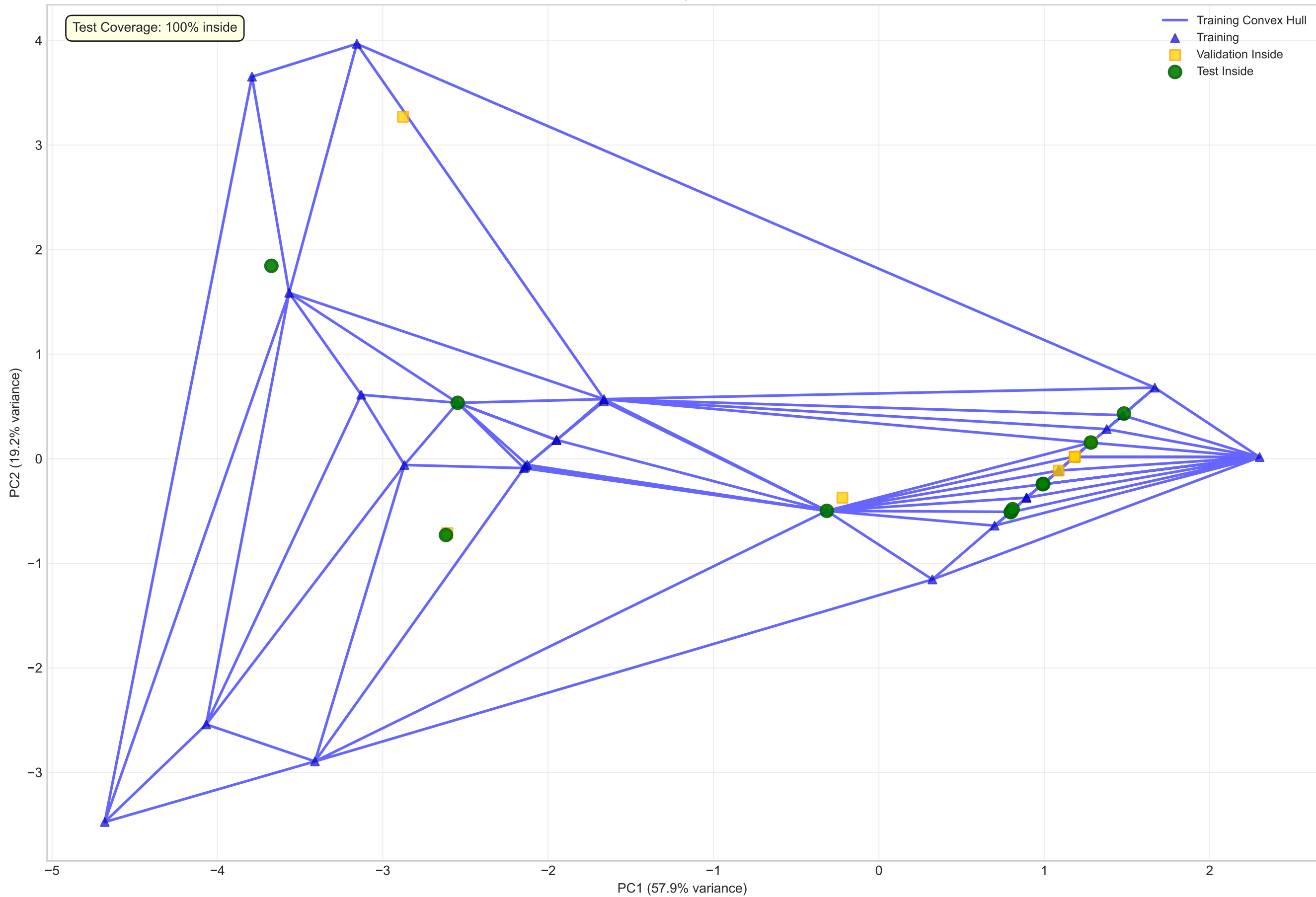
Applicability Domain Analysis Train/Val/Test: 56/9/11 | 11/11 Test Inside Hull
