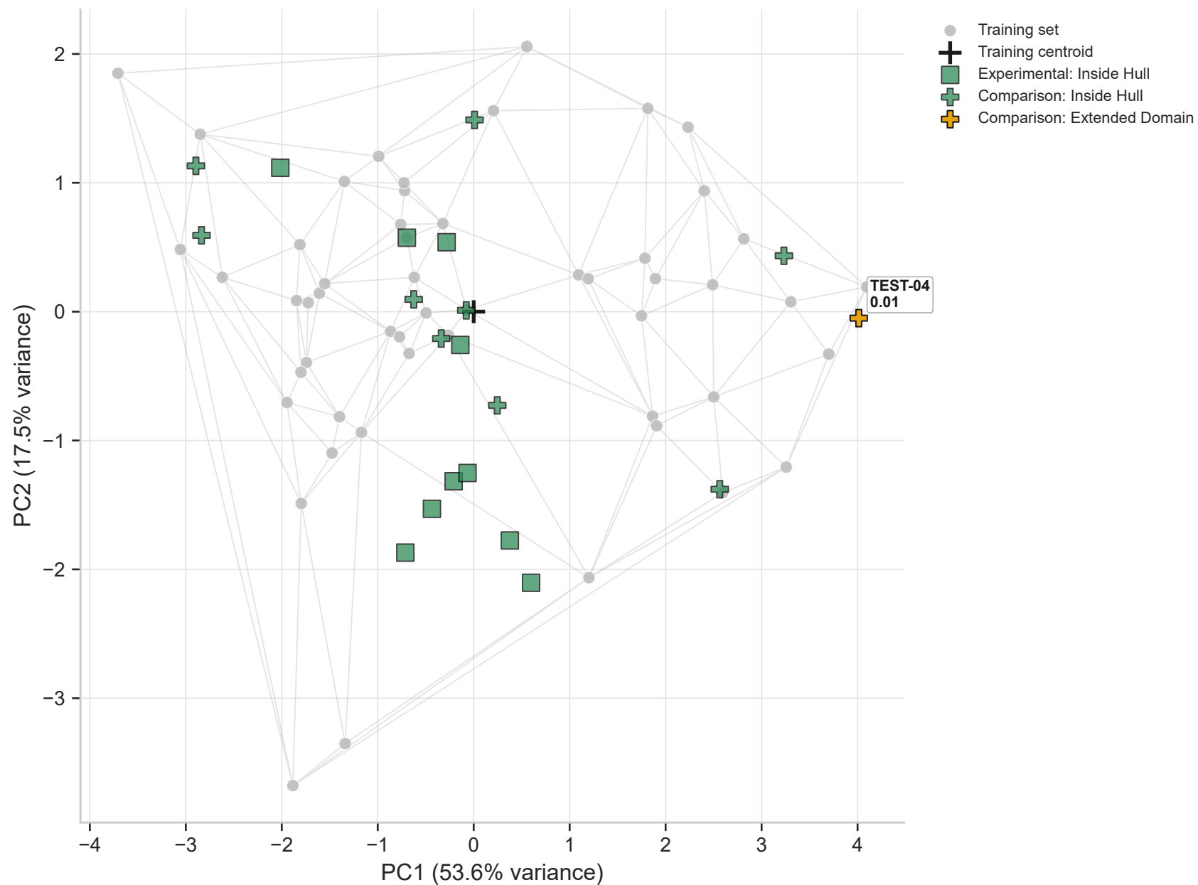
PCA-based applicability-domain visualization (threshold = 0.10)
