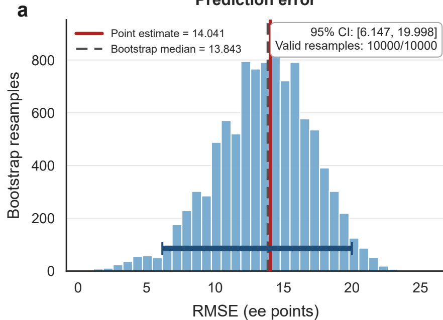
Prediction error
