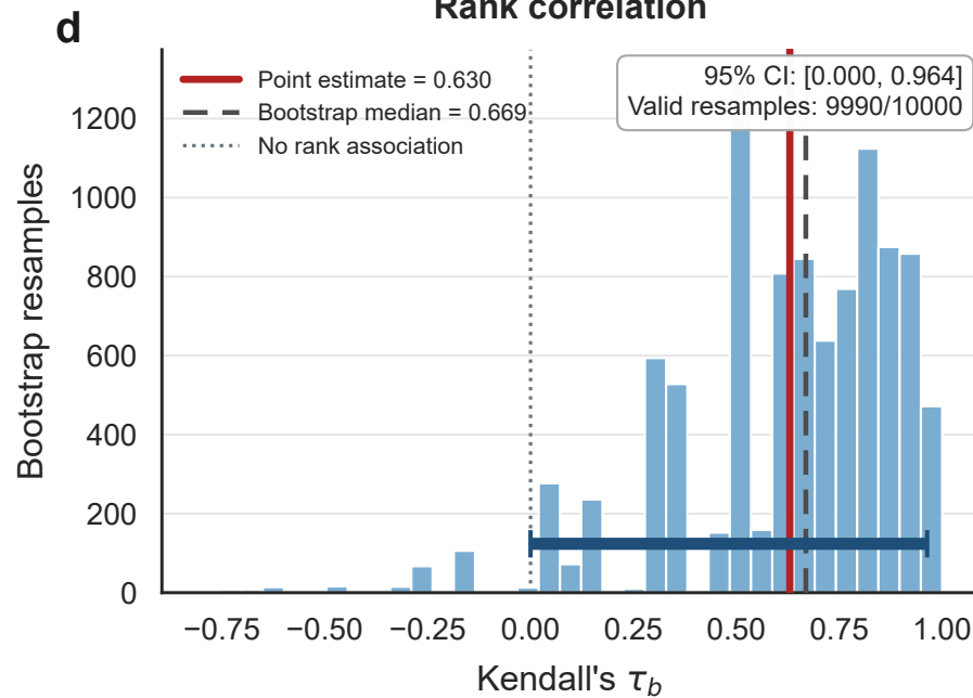
Rank correlation
