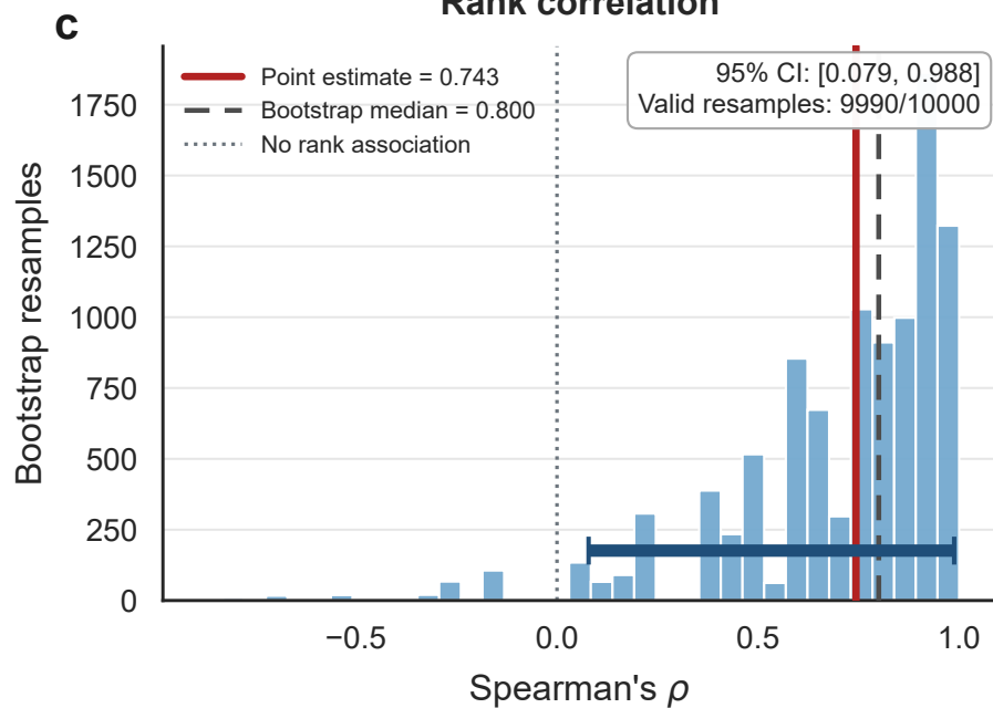
Rank correlation
