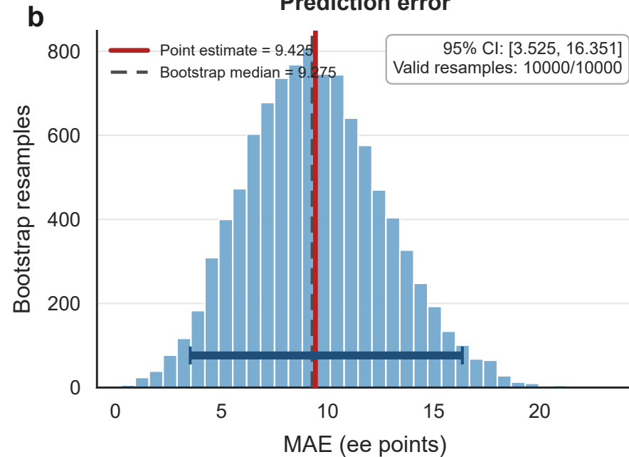
Prediction error
