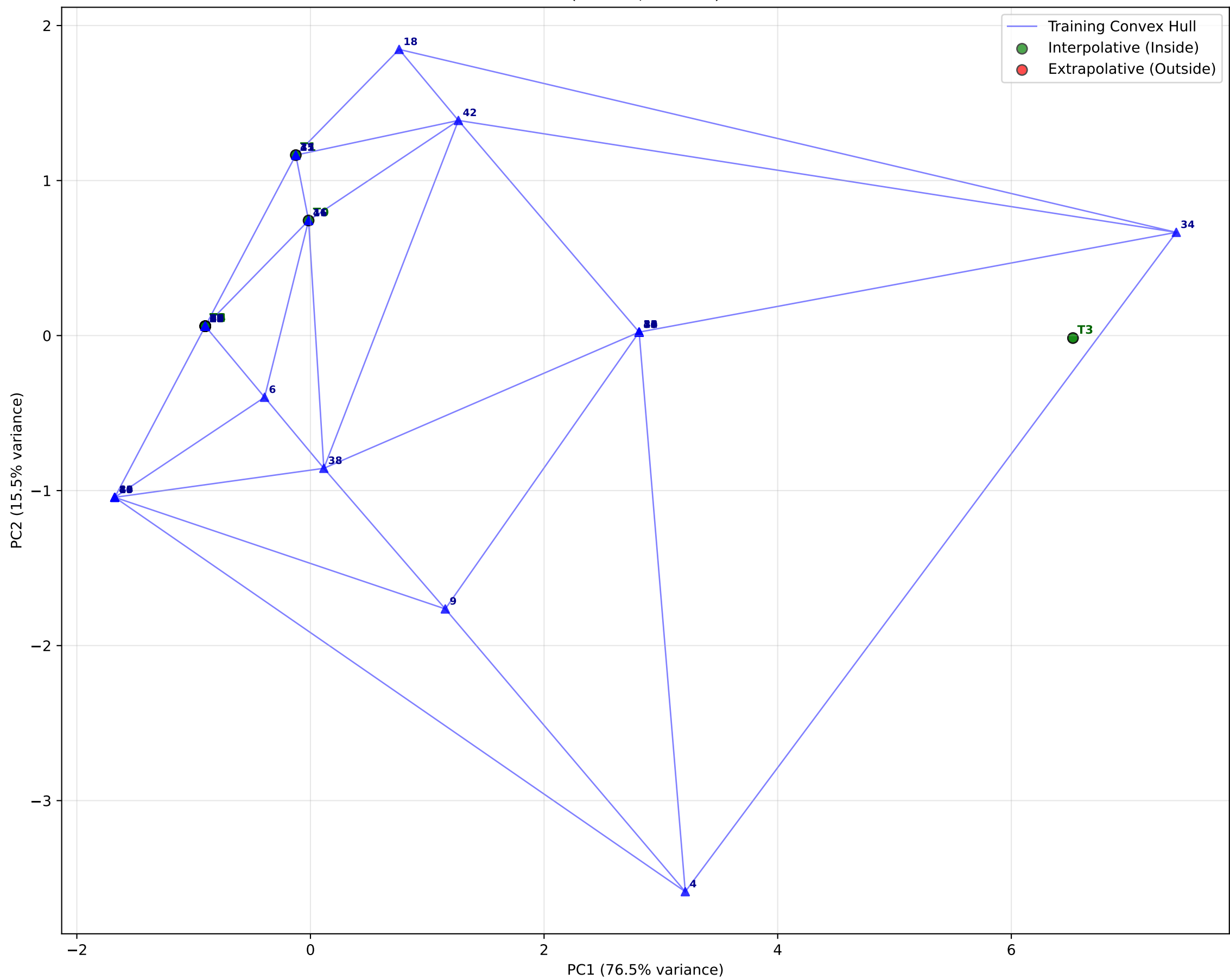
Applicability Domain: Delaunay Triangulation in PCA Space (Train #, Test T#)
