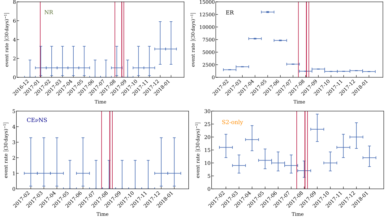
FIG. 2. We show the distribution of background events with time in different analysis channels. Red lines indicate the time of GW events.
