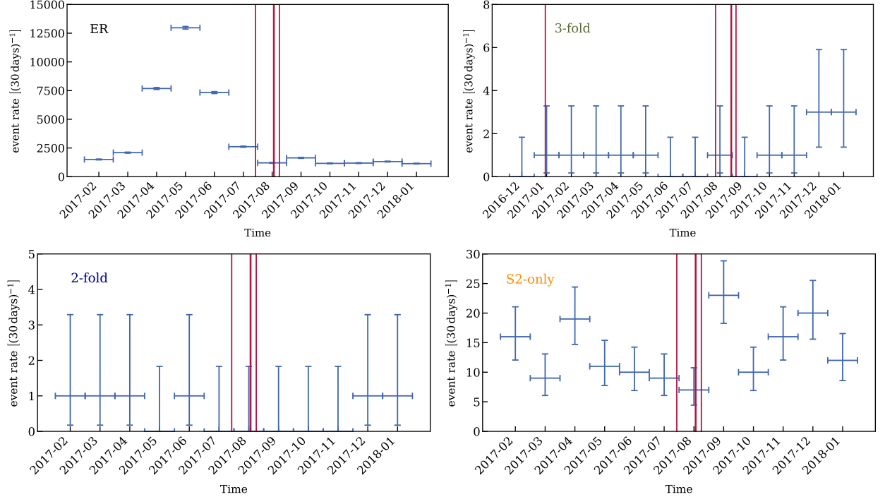
FIG. 2. The distribution of background events with time in ER and NR channels. 3-fold, 2-fold, and S2-only refer to different analysis modes of the NR channel. Red lines indicate the time of GW events. The rise and subsequent decay of event rate in the ER channel during March-September are due to production of ^{131\text{m}}\text{Xe} , ^{133}\text{Xe} , and ^{125}\text{I} during neutron calibration campaigns [32].
