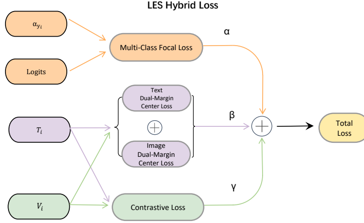
Figure 1: The detailed structure of LES Hybrid Loss.
