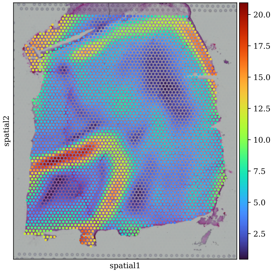
Gradient Boundaries (Slice 151674)
