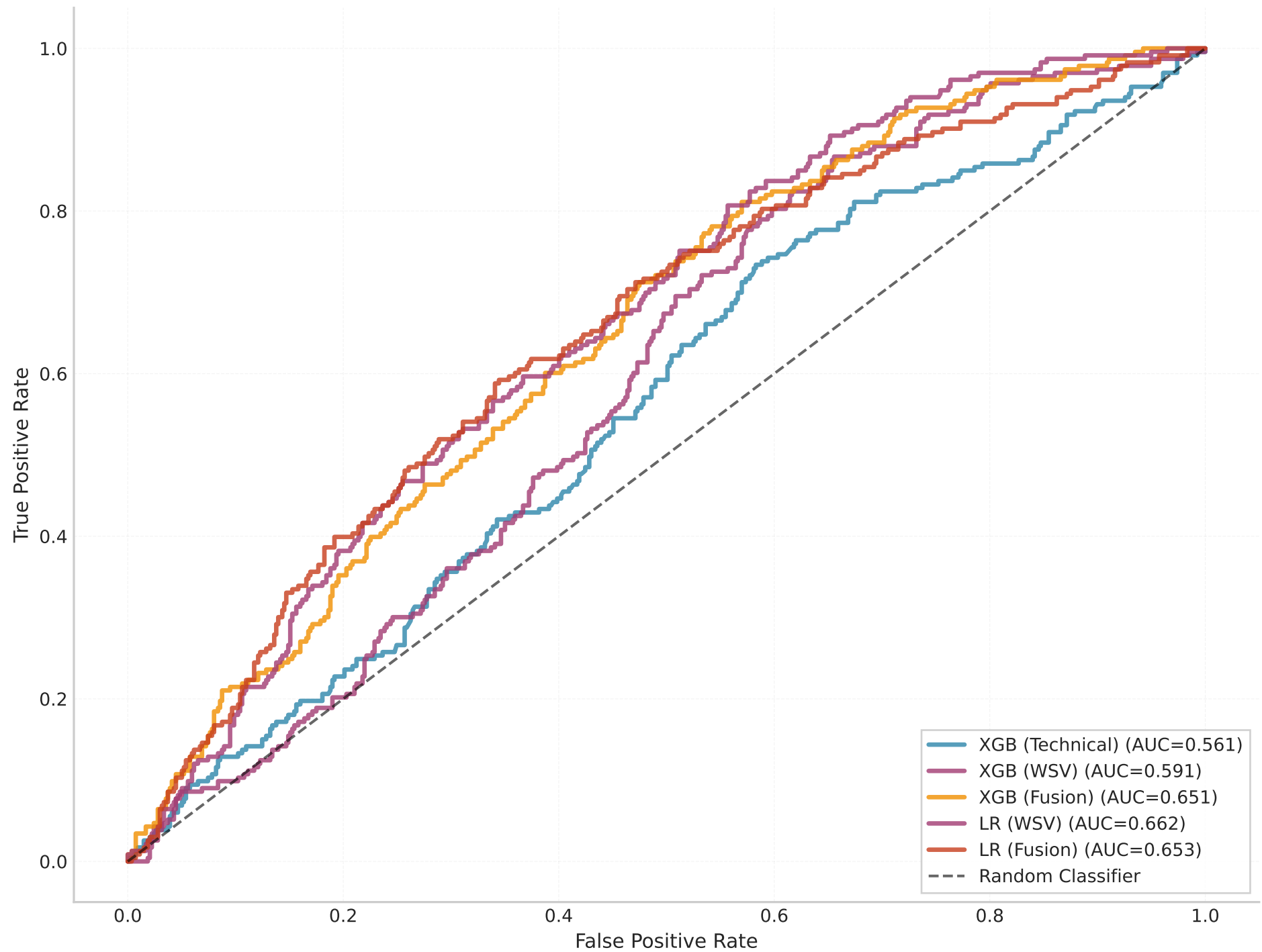
ROC Curves: All Models
