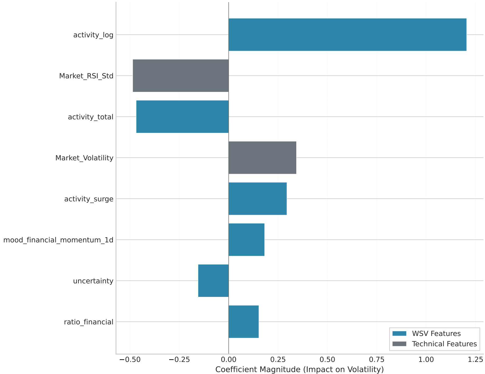
Feature Importance: Logistic Regression (Fusion, RFE Selected)
