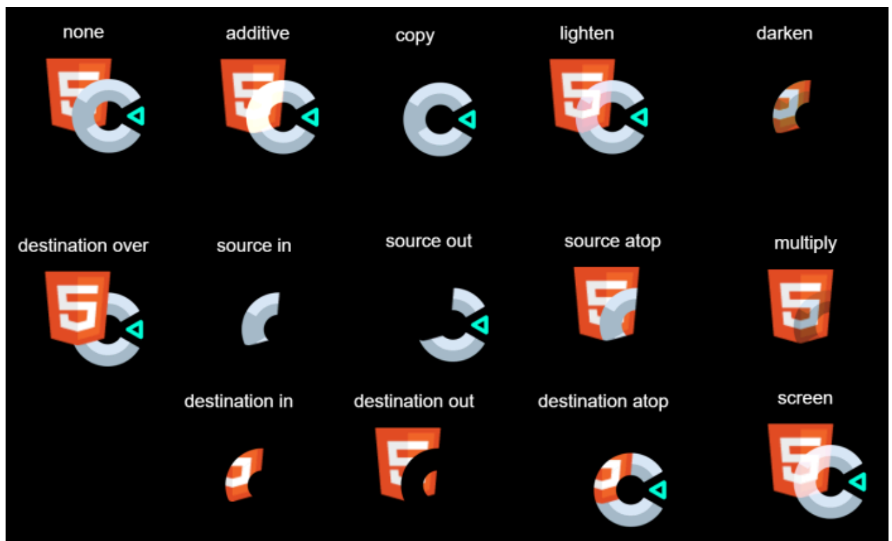
The blend modes available in Construct
