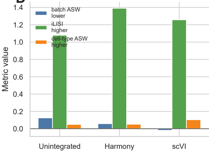
Integration metrics
