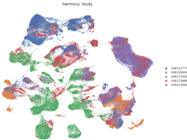
Harmony UMAP by study
