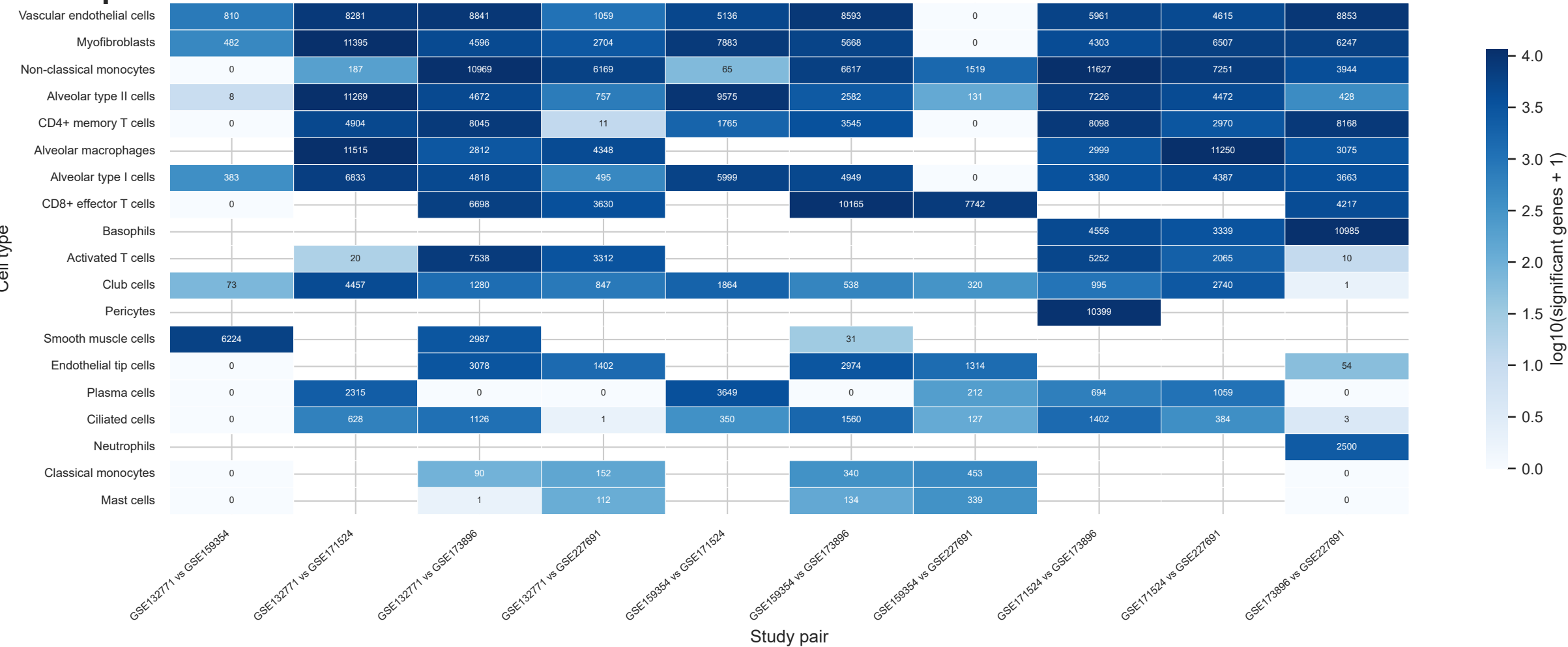
All-study pairwise pseudobulk DE by cell type
