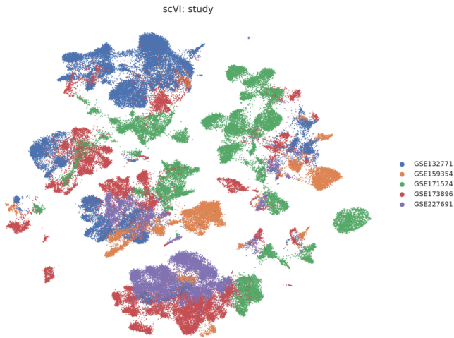
scVI UMAP by study
