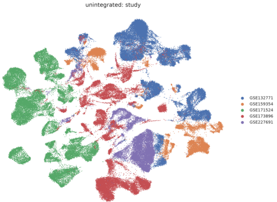
Unintegrated UMAP by study
