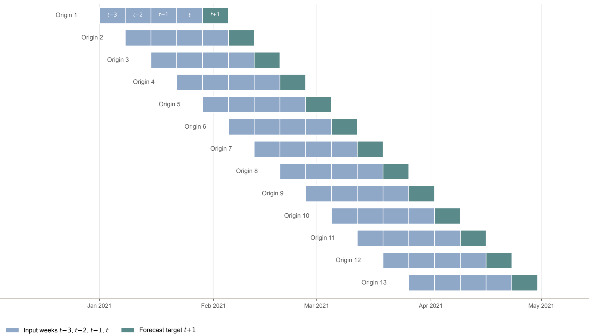
One Fit: testing origin advances one week at a time (13 origins; model held fixed)
