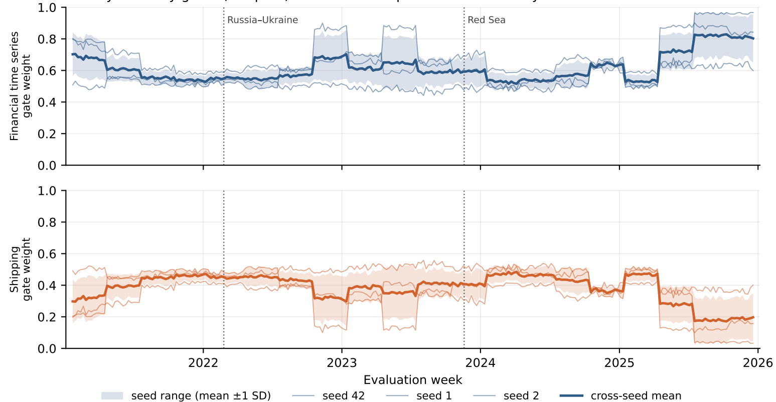
Weekly modality gates (Deep S3): week-to-week paths differ markedly across seeds
