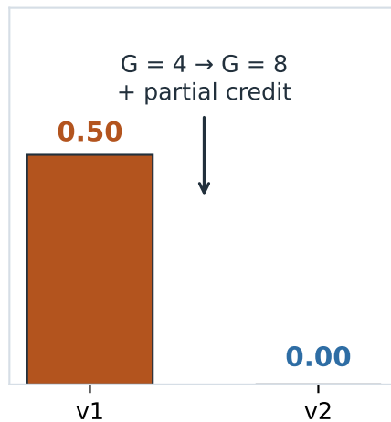
zero-variance GRPO steps
