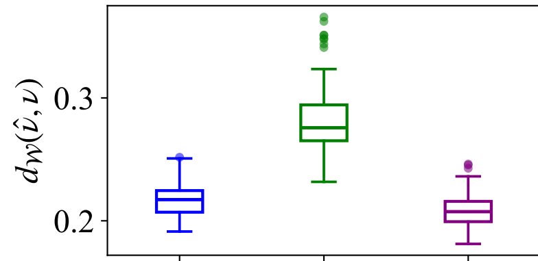
Wasserstein distance
