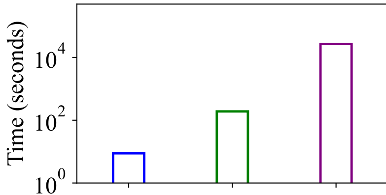
Computational time
