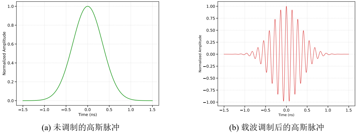
图 3-3 载波调制前后的高斯脉冲, f_c = 7.29\text{GHz} , \text{BW} = 1.4\text{GHz}
