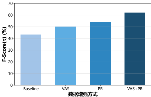
(c) F-Score( \tau ) 对比 (越大越好)
