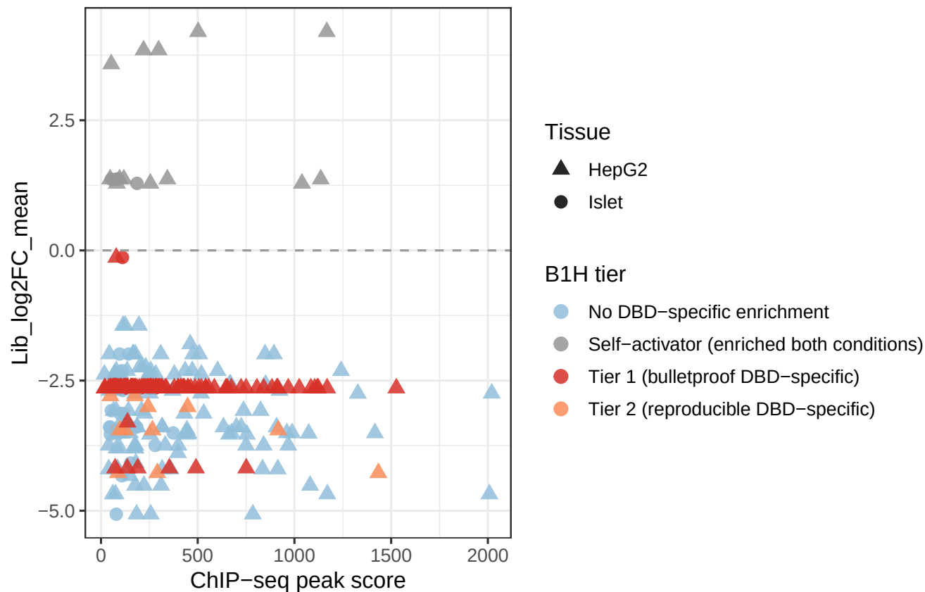
HNF1A Lib_log2FC_mean vs. ChIP-seq peak score 14bp core match ( \pm 3 bp flanking removed)
