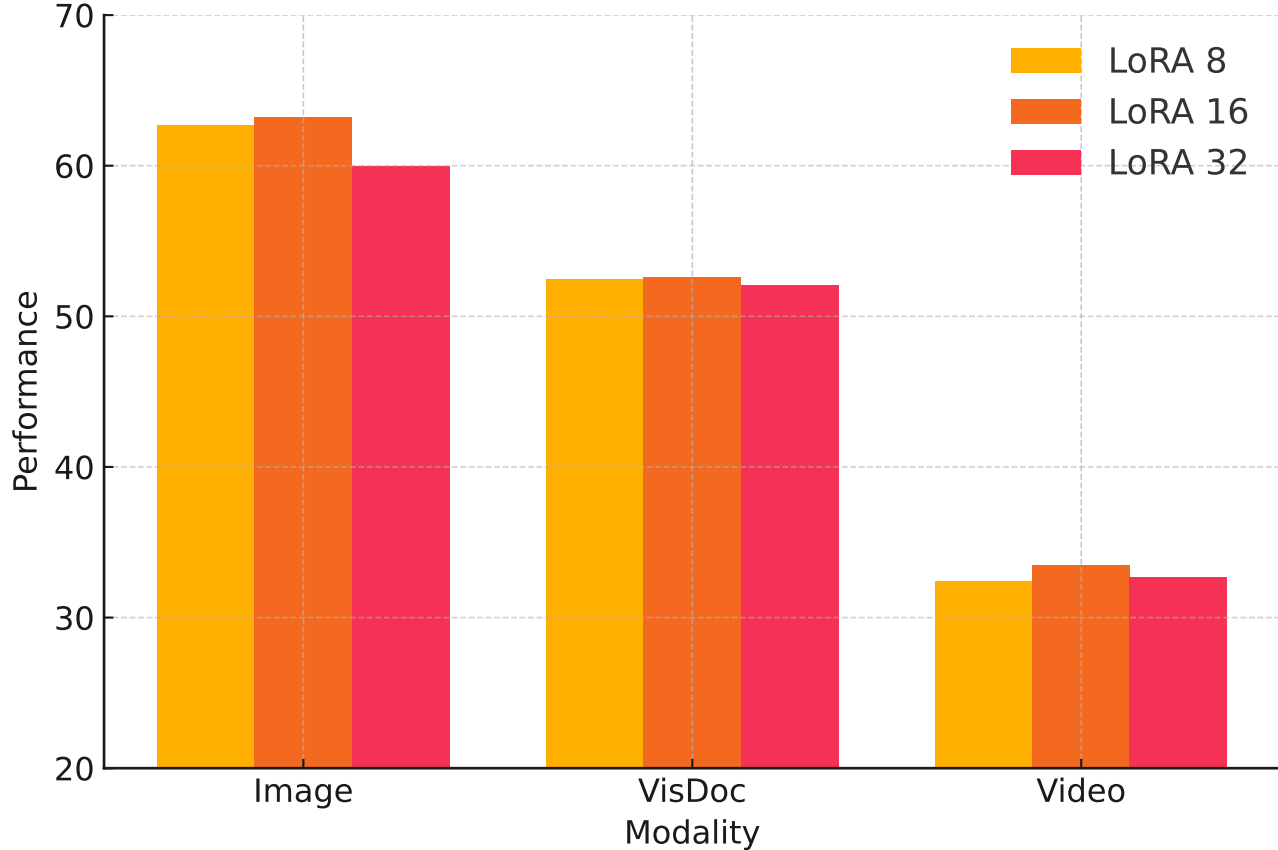
Performance under Different LoRA Ranks
