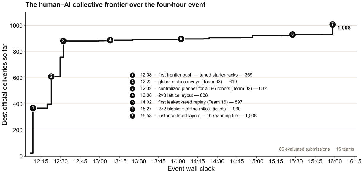
Figure 4. The human-AI collective frontier over the four-hour event. Numbered markers are the milestones of the run, from the first frontier push to the winning instance-fitted layout.
