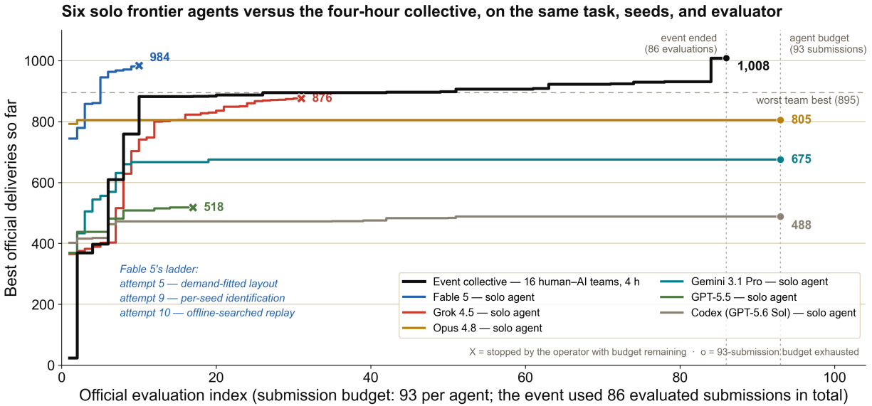
Figure 7. The performance of all six autonomous agents compared to the human collective. Fable 5, unavailable on the day of the event, was the only agent that managed to match the human trajectory by discovering and weaponizing the same exploits.
