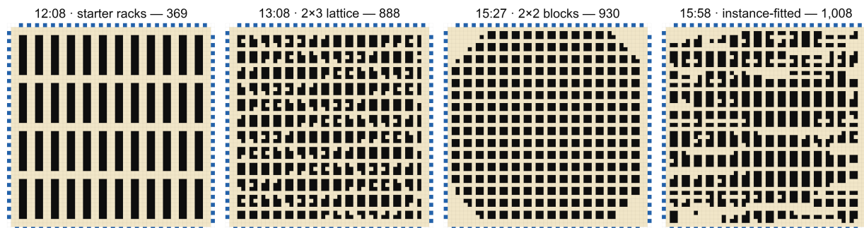
Figure 6. Evolution of the warehouse layout along the human frontier (blue cells are the robots' bases, black cells are shelves). From left to right: the starter long racks (369 deliveries, 12:08), Team 03's 2 \times 3 lattice that opened the layout grind (888, 13:08), Team 10's margin-1 2 \times 2 islands (930, 15:27), and the winning instance-fitted layout optimized offline against the leaked seeds (1,008, 15:58).
