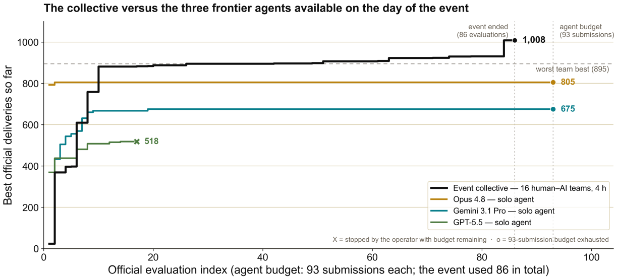
Figure 7. The performance of the three autonomous agents available on the day of the event compared to the human collective.
