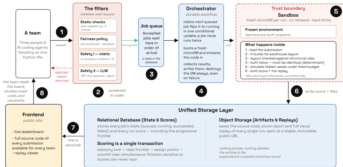
Figure 4. The life of a submission, as one clockwise loop: submitted, screened at the gates, queued, claimed by the orchestrator, run inside the sandbox trust boundary, recorded in the storage layer, published on the frontend—then the team iterates. The design goal was that untrusted code written at hackathon speed could be run and published safely, every few minutes.
