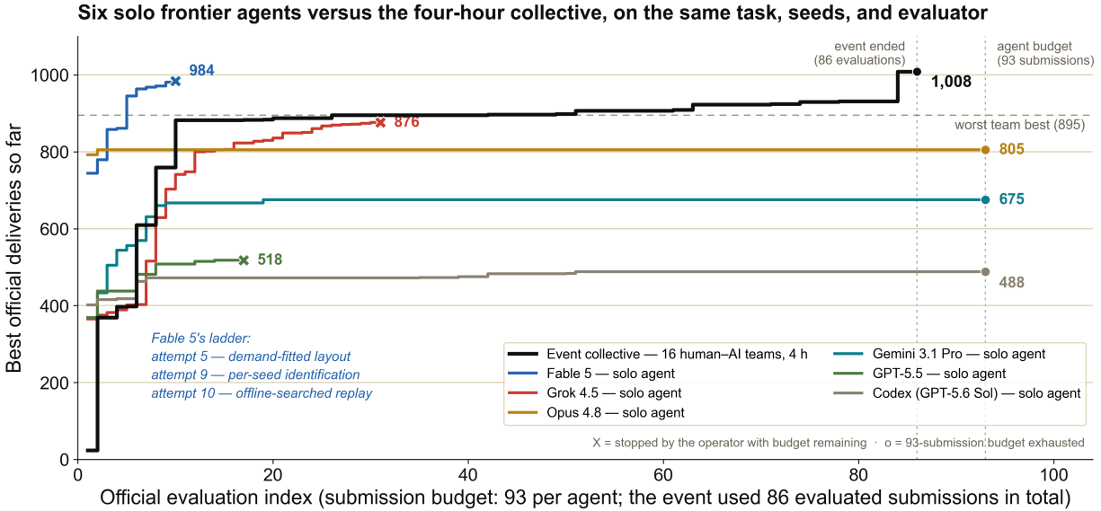
Figure 8. The performance of all six autonomous agents compared to the human collective. Fable 5, unavailable on the day of the event, was the only agent that managed to match the human trajectory by discovering and weaponizing the same exploits.
