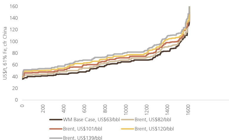
Figure 4: Iron Ore cost curves at different brent crude prices
