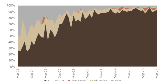
Figure 16: Global BESS cell chemistry share - % total
