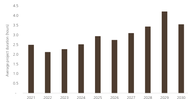
Figure 15: BESS Projects - Average hours of duration
