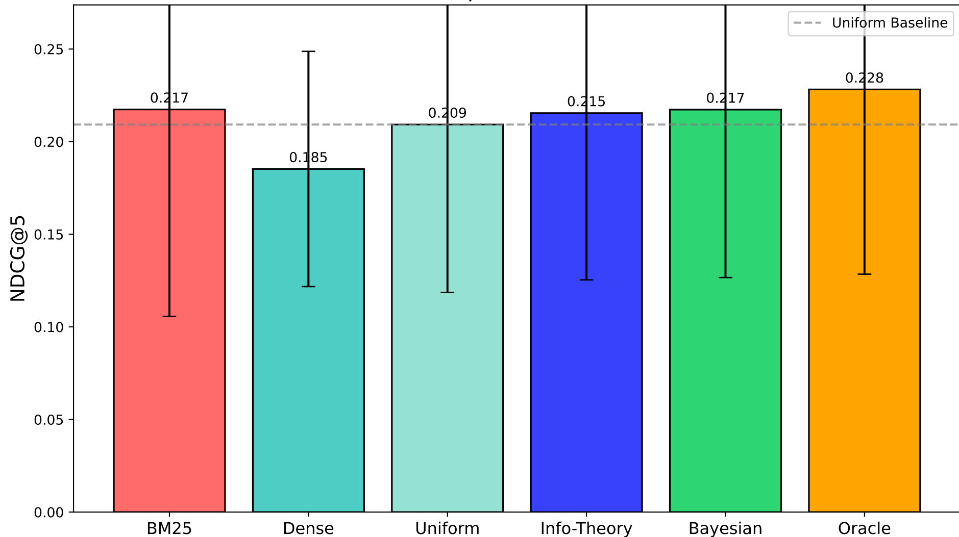
MoRE: Method Comparison on MaintNet Dataset
