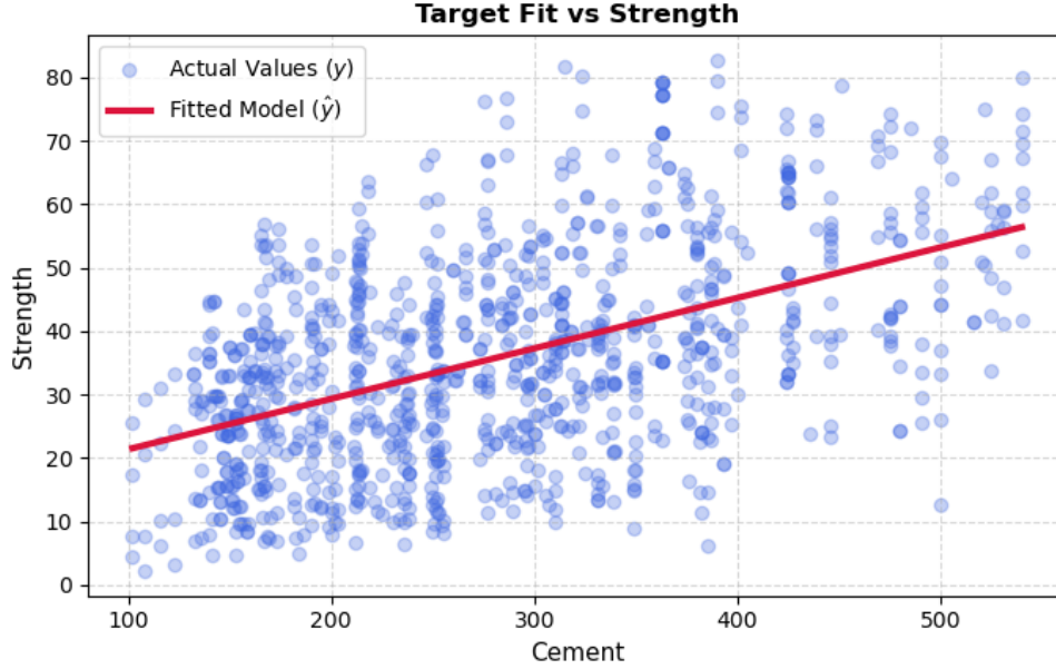
Figure 5: Observed and fitted compressive strength values versus cement.
