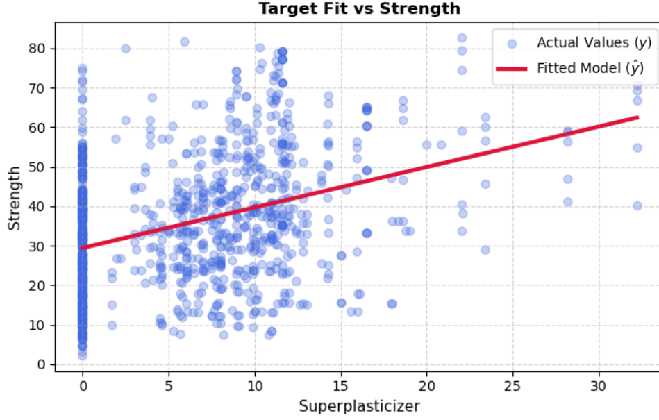
Figure 6: Observed and fitted compressive strength values versus superplasticizer.
