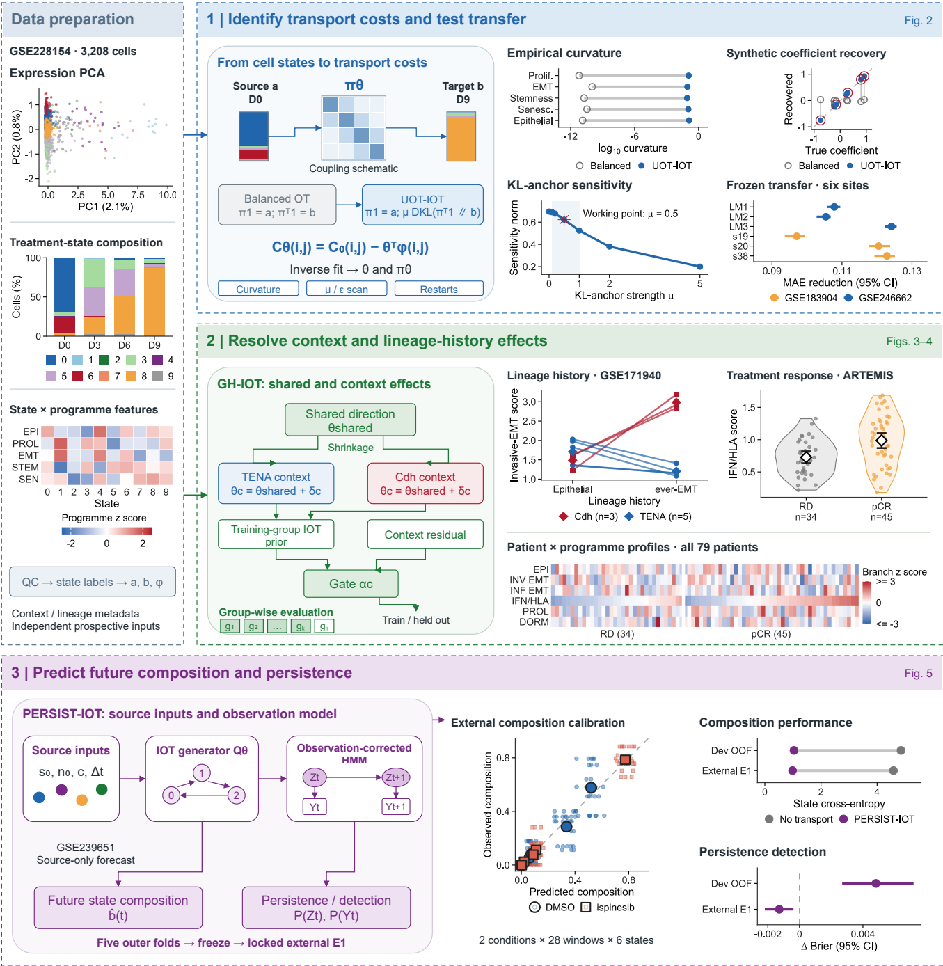
Figure 1 | Technical route for inverse optimal transport
