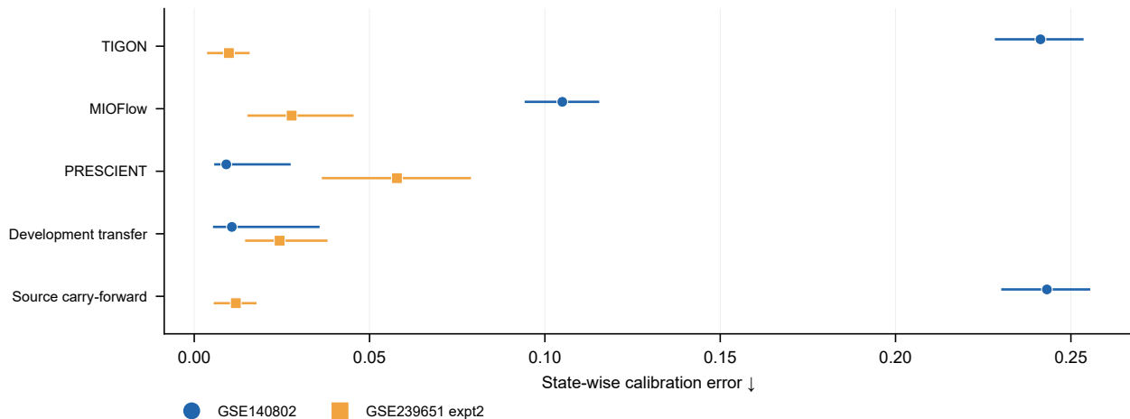
State-wise calibration error with 95% intervals
