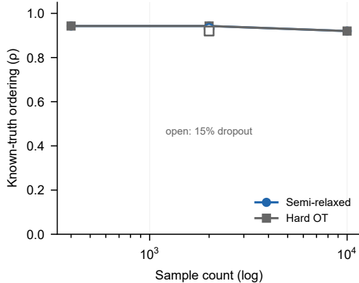
a Known-truth recovery
