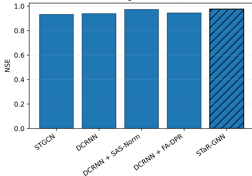
NSE (higher is better)
